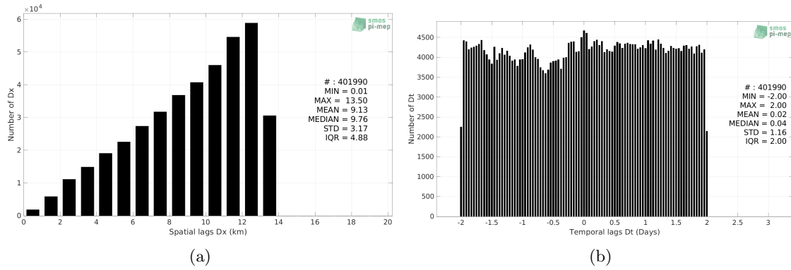
Figure 5: Histograms of the spatial (a) and temporal (b) lags between the location/time of the TSG (GOSUD-Research-vessel) measurement and the date of the corresponding SMAP SSS L4 OI v1 - 7 Days (IPRC) SSS pixel.
