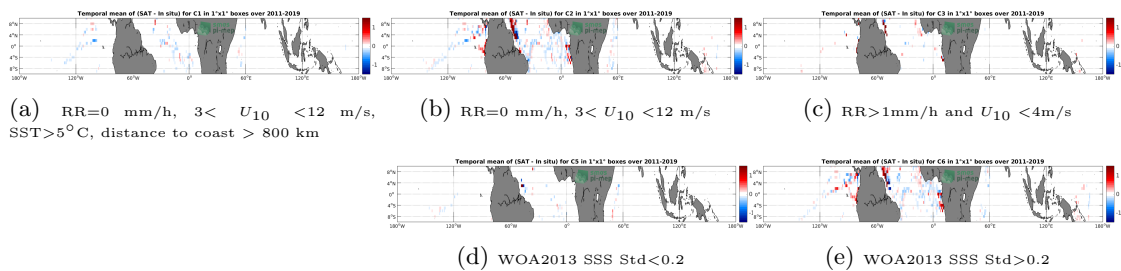
Figure 12: Temporal mean gridded over spatial boxes of size 1^\circ \times 1^\circ of \Delta SSS (SMAP SSS L4 OI v1 - 7day (IPRC) - TSG (GOSUD-Research-vessel)) for 5 different subdatasets corresponding to: RR=0 mm/h, 3 < U_{10} < 12 m/s, SST> 5^\circ\text{C} , distance to coast > 800 km (a), RR=0 mm/h, 3 < U_{10} < 12 m/s (b), RR>1mm/h and U_{10} < 4 m/s (c), WOA2013 SSS Std<0.2 (d), WOA2013 SSS Std>0.2 (e).
