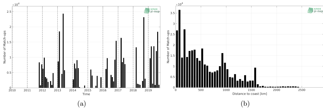
Figure 1: Number of match-ups between TSG (GOSUD-Research-vessel) and SMAP SSS L4 OI v1 - 7day (IPRC) SSS as a function of time (a) and as function of the distance to coast (b) over the Equatorial Ocean 10N-10S Pi-MEP region and for the full satellite product period.
