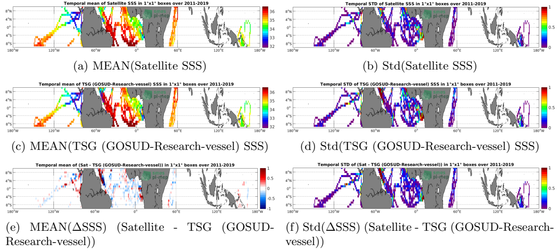
Figure 6: Temporal mean (left) and Std (right) of SSS from SMAP SSS L4 OI v1 - 7day (IPRC) (top), TSG (GOSUD-Research-vessel) (middle), and of \Delta SSS (Satellite - TSG (GOSUD-Research-vessel)). Only match-up pairs are used to generate these maps.
