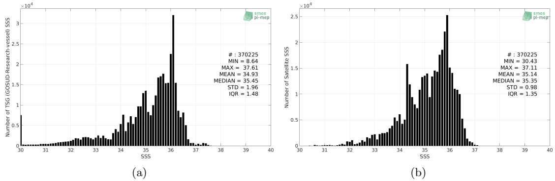
Figure 2: Histograms of SSS from TSG (GOSUD-Research-vessel) (a) and SMAP SSS L4 OI v1 - 7day (IPRC) (b) considering all match-up pairs per bins of 0.1 over the Equatorial Ocean 10N-10S Pi-MEP region and for the full satellite product period.
