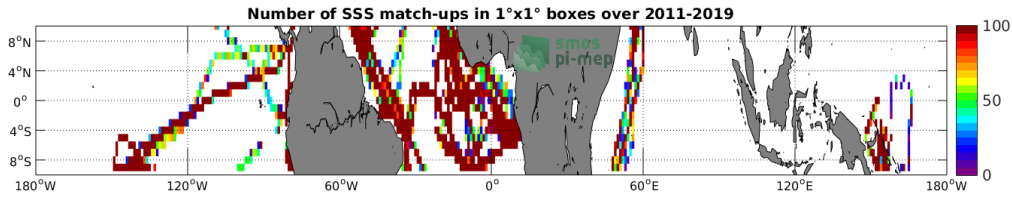
Figure 4: Number of SSS match-ups between TSG (GOSUD-Research-vessel) SSS and the SMAP SSS L4 OI v1 - 7day (IPRC) SSS product for the Equatorial Ocean 10N-10S Pi-MEP region over 1^\circ \times 1^\circ boxes and for the full satellite product period.
