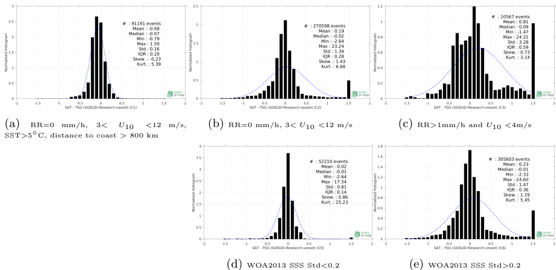
Figure 13: Normalized histogram of \Delta SSS (SMAP SSS L4 OI v1 - 7day (IPRC) - TSG (GOSUD-Research-vessel)) for 5 different subdatasets corresponding to: RR=0 mm/h, 3 < U_{10} < 12 m/s, SST> 5^\circ\text{C} , distance to coast > 800 km (a), RR=0 mm/h, 3 < U_{10} < 12 m/s (b), RR>1mm/h and U_{10} < 4 m/s (c), WOA2013 SSS Std<0.2 (d), WOA2013 SSS Std>0.2 (e).
