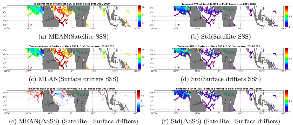
Figure 5: Temporal mean (left) and Std (right) of SSS from SMAP SSS L4 OI v1 - 7day (IPRC) (top), Surface drifters (middle), and of \Delta SSS (Satellite - Surface drifters). Only match-up pairs are used to generate these maps.
