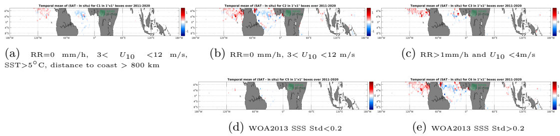
Figure 11: Temporal mean gridded over spatial boxes of size 1°x1° of \Delta SSS (SMAP SSS L4 OI v1 - 7day (IPRC) - Surface drifters) for 5 different subdatasets corresponding to: RR=0 mm/h, 3 < U_{10} < 12 m/s, SST>5°C, distance to coast > 800 km (a), RR=0 mm/h, 3 < U_{10} < 12 m/s (b), RR>1mm/h and U_{10} < 4m/s (c), WOA2013 SSS Std<0.2 (d), WOA2013 SSS Std>0.2 (e).
