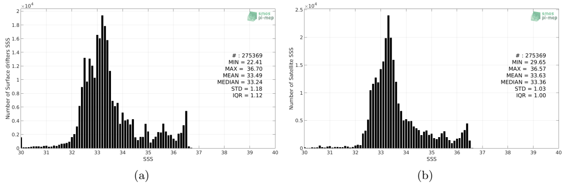
Figure 2: Histograms of SSS from Surface drifters (a) and SMAP SSS L4 OI v1 - 7day (IPRC) (b) considering all match-up pairs per bins of 0.1 over the Equatorial Ocean 10N-10S Pi-MEP region and for the full satellite product period.
