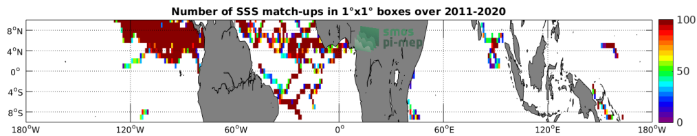
Figure 3: Number of SSS match-ups between Surface drifters SSS and the SMAP SSS L4 OI v1 - 7day (IPRC) SSS product for the Equatorial Ocean 10N-10S Pi-MEP region over 1^\circ \times 1^\circ boxes and for the full satellite product period.
