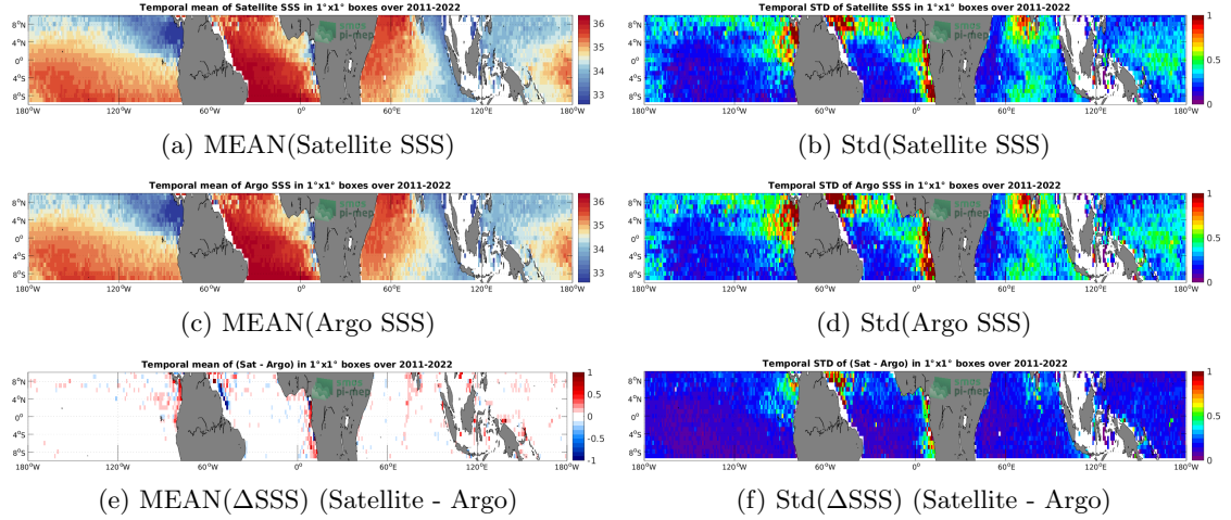
Figure 6: Temporal mean (left) and Std (right) of SSS from SMAP SSS L4 OI v1 - 7 Days (IPRC) (top), Argo (middle), and of \Delta SSS (Satellite - Argo). Only match-up pairs are used to generate these maps.
