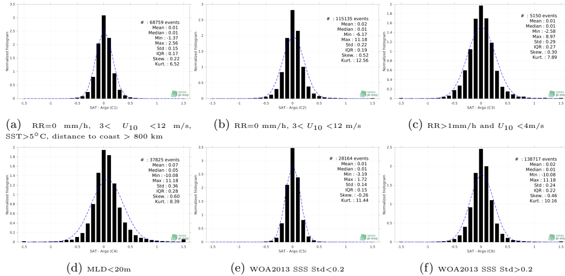
Figure 13: Normalized histogram of \Delta SSS (SMAP SSS L4 OI v1 - 7 Days (IPRC) - Argo) for 6 different subdatasets corresponding to: RR=0 mm/h, 3 < U_{10} < 12 m/s, SST >5^\circ\text{C} , distance to coast > 800 km (a), RR=0 mm/h, 3 < U_{10} < 12 m/s (b), RR >1 mm/h and U_{10} < 4 m/s (c), MLD <20 m (d), WOA2013 SSS Std <0.2 (e), WOA2013 SSS Std >0.2 (f).
