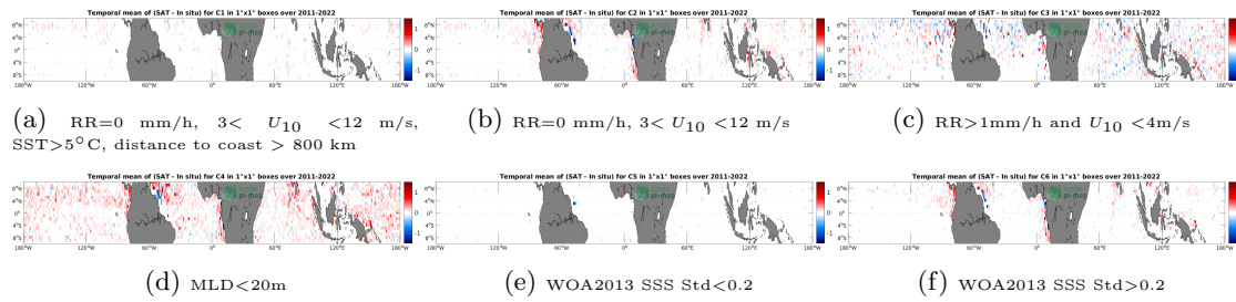
Figure 12: Temporal mean gridded over spatial boxes of size 1^\circ \times 1^\circ of \Delta SSS (SMAP SSS L4 OI v1 - 7 Days (IPRC) - Argo) for 6 different subdatasets corresponding to:RR=0 mm/h, 3 < U_{10} < 12 m/s, SST >5^\circ\text{C} , distance to coast > 800 km (a), RR=0 mm/h, 3 < U_{10} < 12 m/s (b), RR >1 mm/h and U_{10} < 4 m/s (c),MLD <20 m (d),WOA2013 SSS Std <0.2 (e),WOA2013 SSS Std >0.2 (f).
