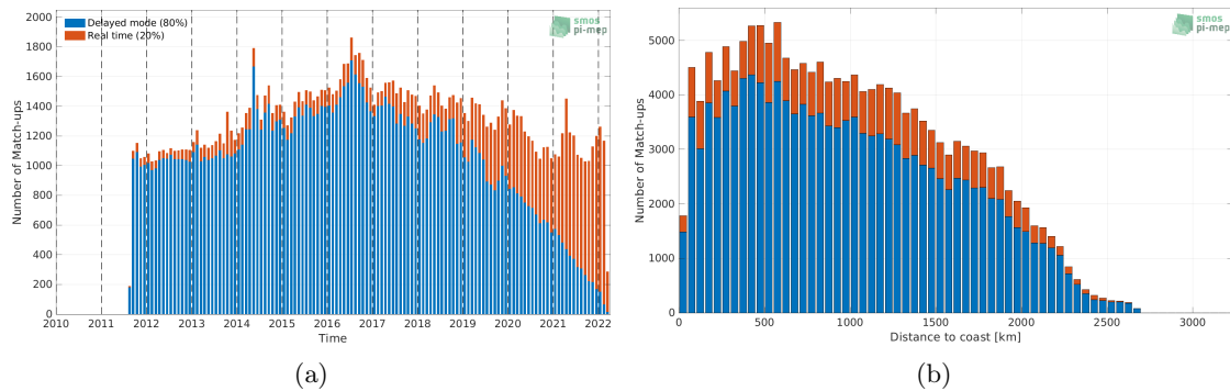
Figure 1: Number of match-ups between Argo and SMAP SSS L4 OI v1 - 7 Days (IPRC) SSS as a function of time (a) and as function of the distance to coast (b) over the Equatorial Ocean 10N-10S Pi-MEP region and for the full satellite product period.
