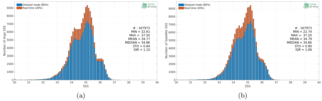
Figure 2: Histograms of SSS from Argo (a) and SMAP SSS L4 OI v1 - 7 Days (IPRC) (b) considering all match-up pairs per bins of 0.1 over the Equatorial Ocean 10N-10S Pi-MEP region and for the full satellite product period.
