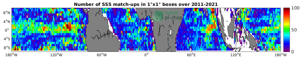
Figure 4: Number of SSS match-ups between Argo SSS and the SMAP SSS L4 OI v1 - 7day (IPRC) SSS product for the Equatorial Ocean 10N-10S Pi-MEP region over 1^\circ \times 1^\circ boxes and for the full satellite product period.
