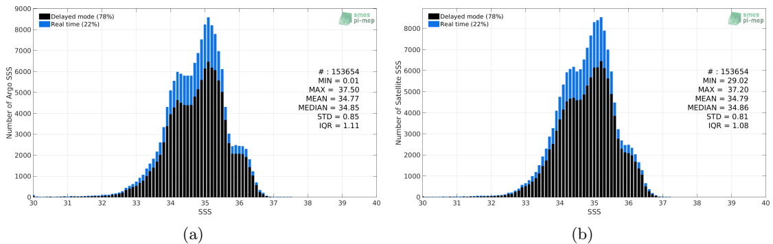
Figure 2: Histograms of SSS from Argo (a) and SMAP SSS L4 OI v1 - 7day (IPRC) (b) considering all match-up pairs per bins of 0.1 over the Equatorial Ocean 10N-10S Pi-MEP region and for the full satellite product period.
