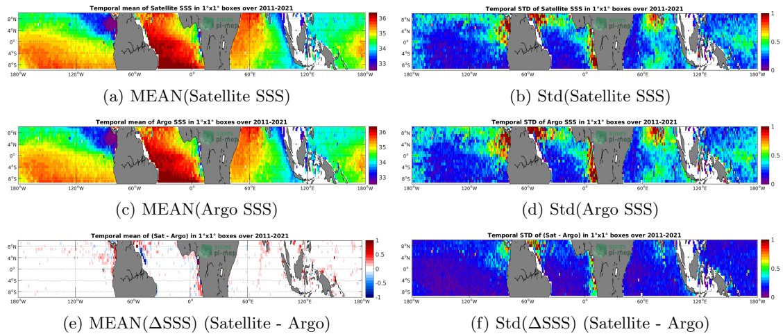
Figure 6: Temporal mean (left) and Std (right) of SSS from SMAP SSS L4 OI v1 - 7day (IPRC) (top), Argo (middle), and of \Delta SSS (Satellite - Argo). Only match-up pairs are used to generate these maps.
