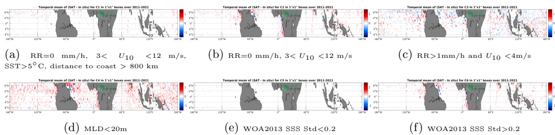
Figure 12: Temporal mean gridded over spatial boxes of size 1°x1° of \Delta SSS (SMAP SSS L4 OI v1 - 7day (IPRC) - Argo) for 6 different subdatasets corresponding to:RR=0 mm/h, 3 < U_{10} < 12 m/s, SST>5°C, distance to coast > 800 km (a), RR=0 mm/h, 3 < U_{10} < 12 m/s (b), RR>1mm/h and U_{10} <4m/s (c),MLD<20m (d),WOA2013 SSS Std<0.2 (e),WOA2013 SSS Std>0.2 (f).
