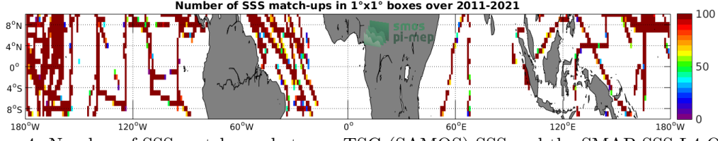
Figure 4: Number of SSS match-ups between TSG (SAMOS) SSS and the SMAP SSS L4 OI v1 - Monthly (IPRC) SSS product for the Equatorial Ocean 10N-10S Pi-MEP region over 1^\circ \times 1^\circ boxes and for the full satellite product period.
