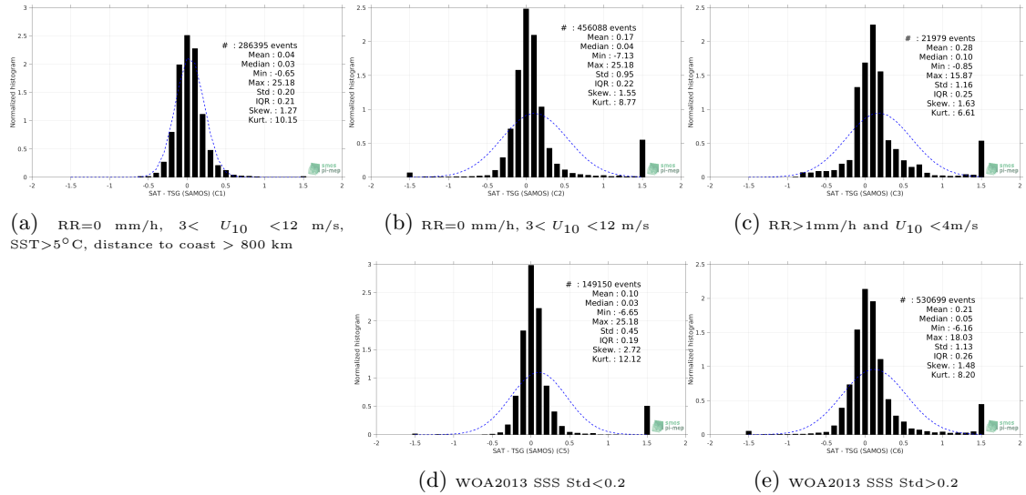
Figure 13: Normalized histogram of \Delta SSS (SMAP SSS L4 OI v1 - Monthly (IPRC) - TSG (SAMOS)) for 5 different subdatasets corresponding to: RR=0 mm/h, 3 < U_{10} < 12 m/s, SST > 5^\circ C , distance to coast > 800 km (a), RR=0 mm/h, 3 < U_{10} < 12 m/s (b), RR > 1 mm/h and U_{10} < 4 m/s (c), WOA2013 SSS Std < 0.2 (d), WOA2013 SSS Std > 0.2 (e).
