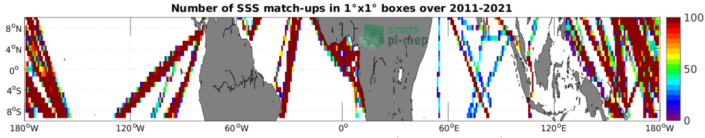
Figure 4: Number of SSS match-ups between TSG (LEGOS-DM) SSS and the SMAP SSS L4 OI v1 - Monthly (IPRC) SSS product for the Equatorial Ocean 10N-10S Pi-MEP region over 1^\circ \times 1^\circ boxes and for the full satellite product period.
