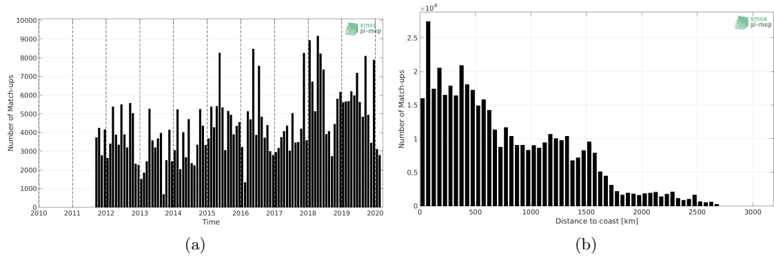
Figure 1: Number of match-ups between TSG (LEGOS-DM) and SMAP SSS L4 OI v1 - Monthly (IPRC) SSS as a function of time (a) and as function of the distance to coast (b) over the Equatorial Ocean 10N-10S Pi-MEP region and for the full satellite product period.
