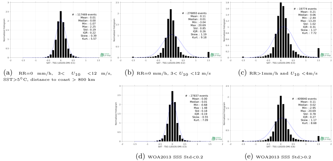
Figure 13: Normalized histogram of \Delta SSS (SMAP SSS L4 OI v1 - Monthly (IPRC) - TSG (LEGOS-DM)) for 5 different subdatasets corresponding to: RR=0 mm/h, 3 < U_{10} < 12 m/s, SST >5^\circ\text{C} , distance to coast > 800 km (a), RR=0 mm/h, 3 < U_{10} < 12 m/s (b), RR >1 mm/h and U_{10} < 4 m/s (c), WOA2013 SSS Std <0.2 (d), WOA2013 SSS Std >0.2 (e).
