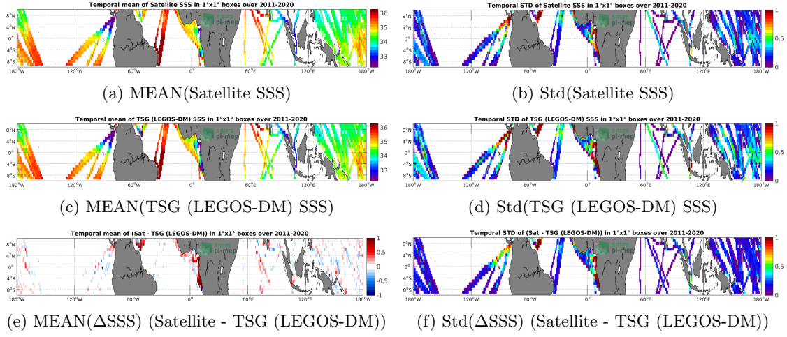
Figure 6: Temporal mean (left) and Std (right) of SSS from SMAP SSS L4 OI v1 - Monthly (IPRC) (top), TSG (LEGOS-DM) (middle), and of \Delta SSS (Satellite - TSG (LEGOS-DM)). Only match-up pairs are used to generate these maps.
