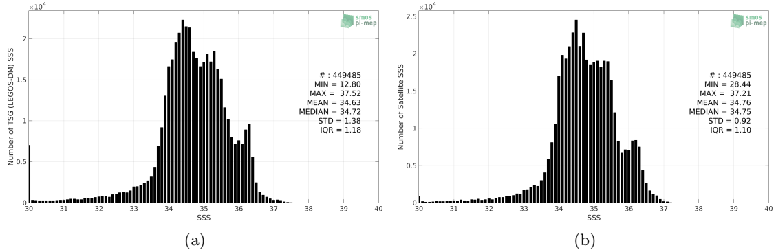
Figure 2: Histograms of SSS from TSG (LEGOS-DM) (a) and SMAP SSS L4 OI v1 - Monthly (IPRC) (b) considering all match-up pairs per bins of 0.1 over the Equatorial Ocean 10N-10S Pi-MEP region and for the full satellite product period.
