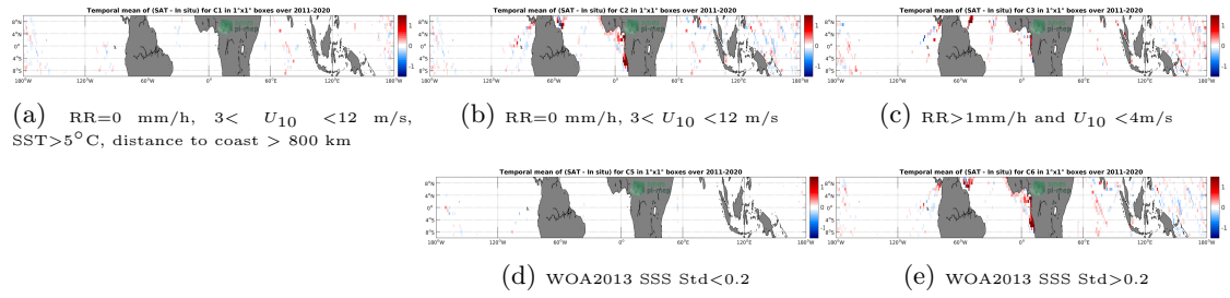
Figure 12: Temporal mean gridded over spatial boxes of size 1^\circ \times 1^\circ of \Delta SSS (SMAP SSS L4 OI v1 - Monthly (IPRC) - TSG (LEGOS-DM)) for 5 different subdatasets corresponding to: RR=0 mm/h, 3 < U_{10} < 12 m/s, SST >5^\circ\text{C} , distance to coast > 800 km (a), RR=0 mm/h, 3 < U_{10} < 12 m/s (b), RR >1 mm/h and U_{10} < 4 m/s (c), WOA2013 SSS Std <0.2 (d), WOA2013 SSS Std >0.2 (e).
