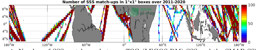
Figure 4: Number of SSS match-ups between TSG (LEGOS-DM) SSS and the SMAP SSS L4 OI v1 - Monthly (IPRC) SSS product for the Equatorial Ocean 10N-10S Pi-MEP region over 1^\circ \times 1^\circ boxes and for the full satellite product period.
