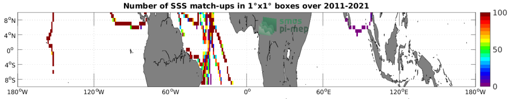
Figure 4: Number of SSS match-ups between TSG (GOSUD-Sailing-ship) SSS and the SMAP SSS L4 OI v1 - Monthly (IPRC) SSS product for the Equatorial Ocean 10N-10S Pi-MEP region over 1^\circ \times 1^\circ boxes and for the full satellite product period.
