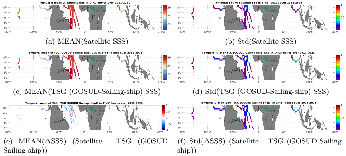
Figure 6: Temporal mean (left) and Std (right) of SSS from SMAP SSS L4 OI v1 - Monthly (IPRC) (top), TSG (GOSUD-Sailing-ship) (middle), and of \Delta SSS (Satellite - TSG (GOSUD-Sailing-ship)). Only match-up pairs are used to generate these maps.
