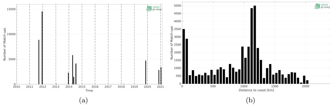
Figure 1: Number of match-ups between TSG (GOSUD-Sailing-ship) and SMAP SSS L4 OI v1 - Monthly (IPRC) SSS as a function of time (a) and as function of the distance to coast (b) over the Equatorial Ocean 10N-10S Pi-MEP region and for the full satellite product period.
