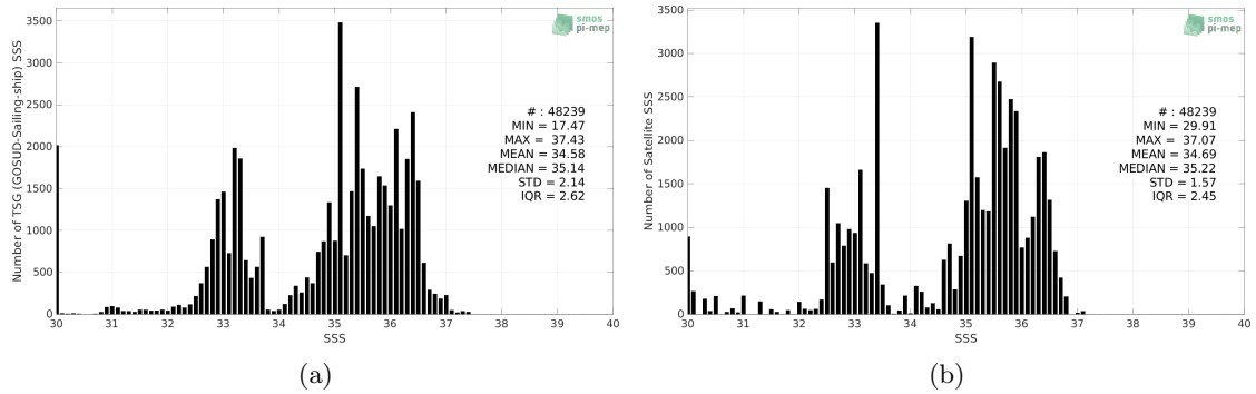
Figure 2: Histograms of SSS from TSG (GOSUD-Sailing-ship) (a) and SMAP SSS L4 OI v1 - Monthly (IPRC) (b) considering all match-up pairs per bins of 0.1 over the Equatorial Ocean 10N-10S Pi-MEP region and for the full satellite product period.
