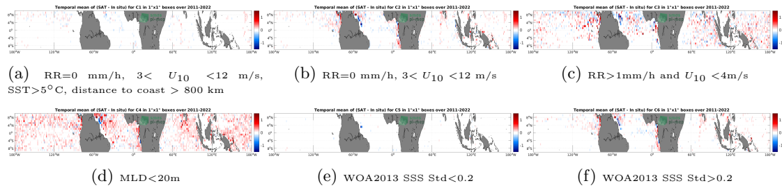
Figure 12: Temporal mean gridded over spatial boxes of size 1^\circ \times 1^\circ of \Delta SSS (SMAP SSS L4 OI v1 - Monthly (IPRC) - Argo) for 6 different subdatasets corresponding to:RR=0 mm/h, 3 < U_{10} < 12 m/s, SST >5^\circ C, distance to coast > 800 km (a), RR=0 mm/h, 3 < U_{10} < 12 m/s (b), RR >1 mm/h and U_{10} < 4 m/s (c),MLD <20 m (d),WOA2013 SSS Std <0.2 (e),WOA2013 SSS Std >0.2 (f).
