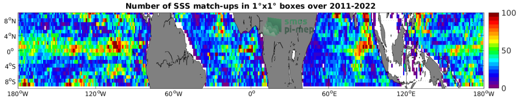
Figure 4: Number of SSS match-ups between Argo SSS and the SMAP SSS L4 OI v1 - Monthly (IPRC) SSS product for the Equatorial Ocean 10N-10S Pi-MEP region over 1^\circ \times 1^\circ boxes and for the full satellite product period.
