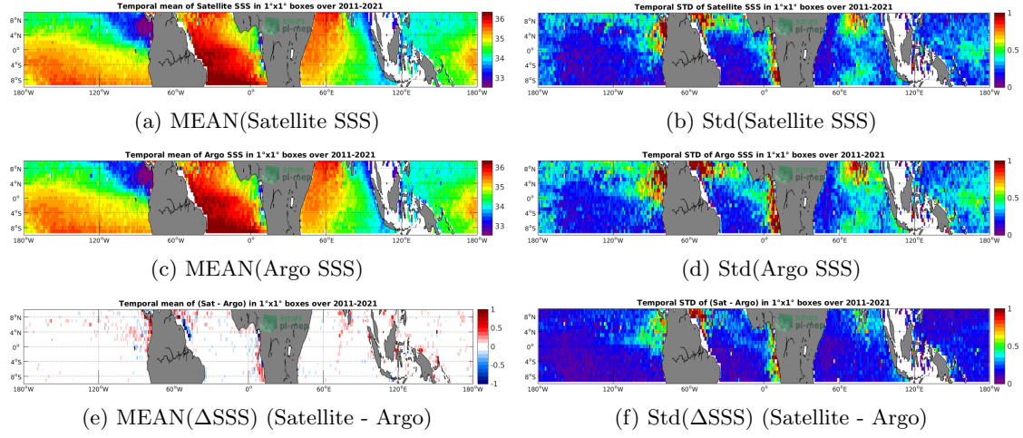
Figure 6: Temporal mean (left) and Std (right) of SSS from SMAP SSS L4 OI v1 - Monthly (IPRC) (top), Argo (middle), and of \Delta SSS (Satellite - Argo). Only match-up pairs are used to generate these maps.
