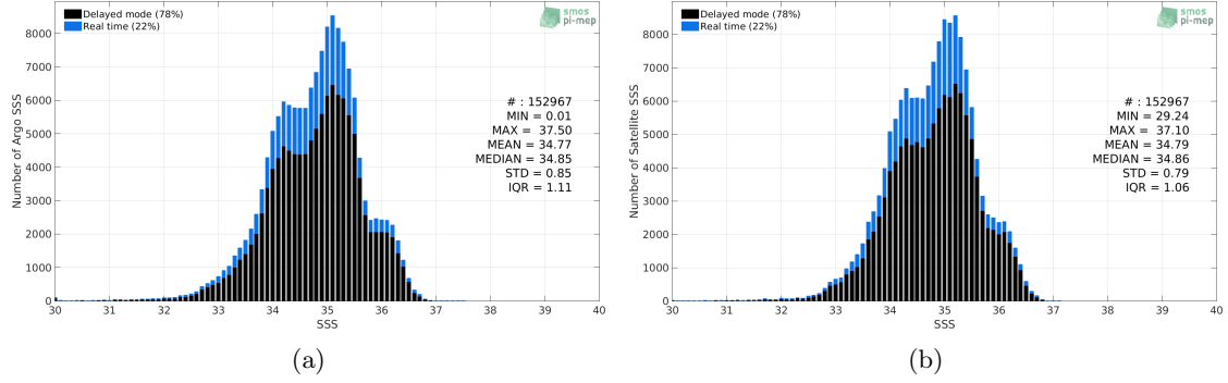
Figure 2: Histograms of SSS from Argo (a) and SMAP SSS L4 OI v1 - Monthly (IPRC) (b) considering all match-up pairs per bins of 0.1 over the Equatorial Ocean 10N-10S Pi-MEP region and for the full satellite product period.
