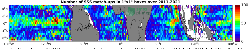
Figure 4: Number of SSS match-ups between Argo SSS and the SMAP SSS L4 OI v1 - Monthly (IPRC) SSS product for the Equatorial Ocean 10N-10S Pi-MEP region over 1^\circ \times 1^\circ boxes and for the full satellite product period.
