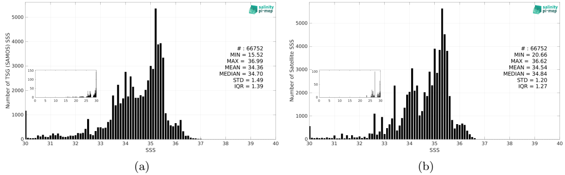
Figure 3: Histograms of SSS from TSG (SAMOS) (a) and SMAP SSS L4 OI v3 - Monthly (ESR) (b) considering all match-up pairs per bins of 0.1 over the Equatorial Ocean 10N-10S Pi-MEP region and for the full satellite product period.
