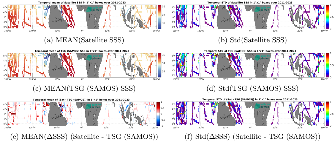
Figure 7: Temporal mean (left) and Std (right) of SSS from SMAP SSS L4 OI v3 - Monthly (ESR) (top), TSG (SAMOS) (middle), and of \Delta SSS (Satellite - TSG (SAMOS)). Only match-up pairs are used to generate these maps.
