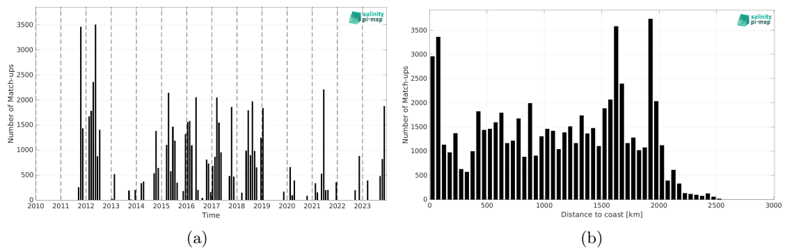
Figure 2: Number of match-ups between TSG (SAMOS) and SMAP SSS L4 OI v3 - Monthly (ESR) SSS as a function of time (a) and as function of the distance to coast (b) over the Equatorial Ocean 10N-10S Pi-MEP region and for the full satellite product period.
