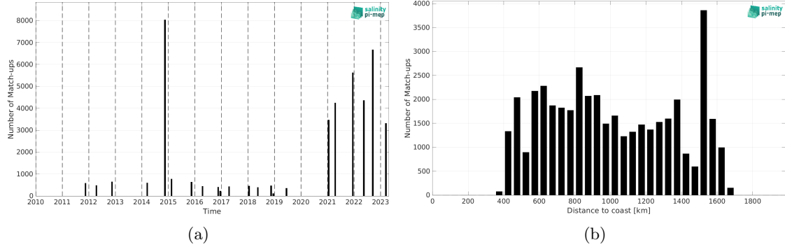
Figure 2: Number of match-ups between TSG (Polarstern) and SMAP SSS L4 OI v3 - Monthly (ESR) SSS as a function of time (a) and as function of the distance to coast (b) over the Equatorial Ocean 10N-10S Pi-MEP region and for the full satellite product period.
