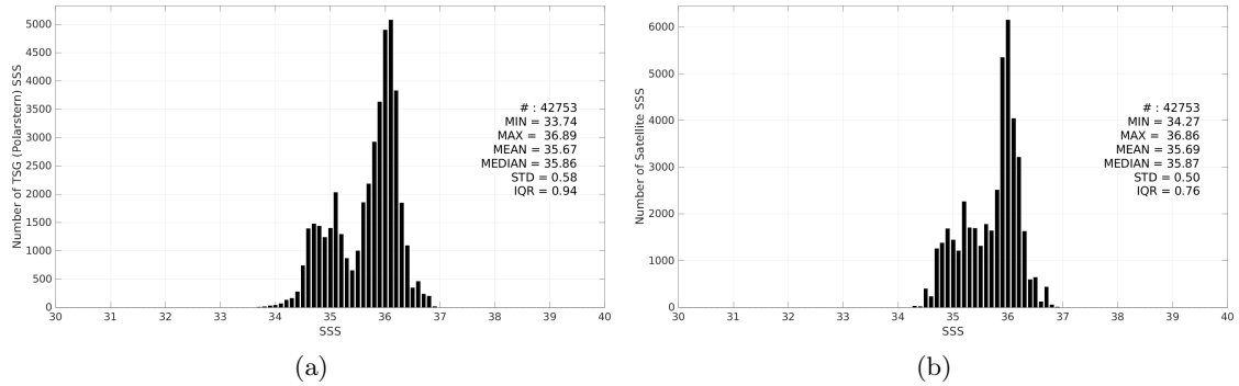
Figure 3: Histograms of SSS from TSG (Polarstern) (a) and SMAP SSS L4 OI v3 - Monthly (ESR) (b) considering all match-up pairs per bins of 0.1 over the Equatorial Ocean 10N-10S Pi-MEP region and for the full satellite product period.
