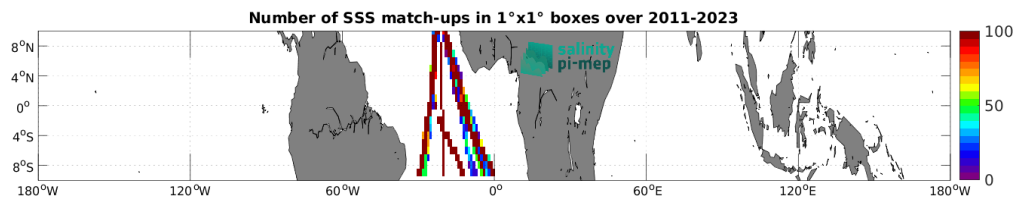
Figure 5: Number of SSS match-ups between TSG (Polarstern) SSS and the SMAP SSS L4 OI v3 - Monthly (ESR) SSS product for the Equatorial Ocean 10N-10S Pi-MEP region over 1^\circ \times 1^\circ boxes and for the full satellite product period.
