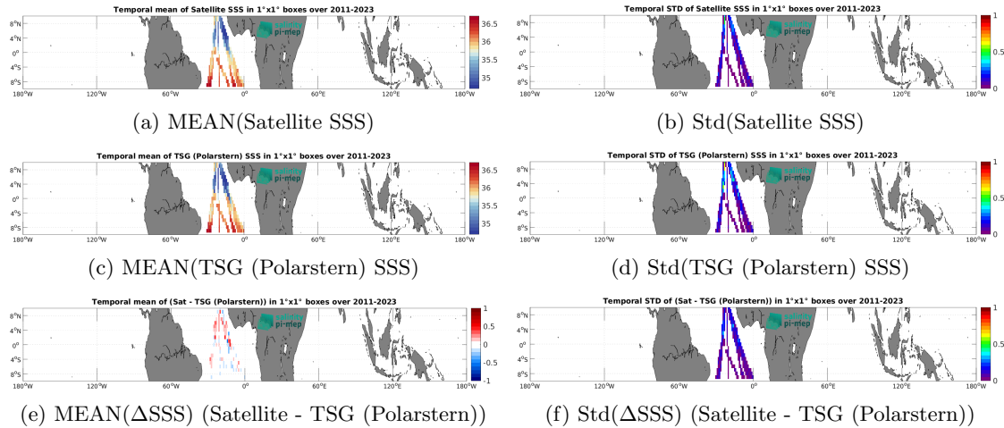
Figure 7: Temporal mean (left) and Std (right) of SSS from SMAP SSS L4 OI v3 - Monthly (ESR) (top), TSG (Polarstern) (middle), and of \Delta SSS (Satellite - TSG (Polarstern)). Only match-up pairs are used to generate these maps.
