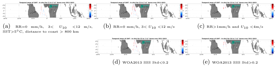
Figure 14: Temporal mean gridded over spatial boxes of size 1^\circ \times 1^\circ of \Delta SSS (SMAP SSS L4 OI v3 - Monthly (ESR) - TSG (Polarstern)) for 5 different subdatasets corresponding to: RR=0 mm/h, 3 < U_{10} < 12 m/s, SST>5°C, distance to coast > 800 km (a), RR=0 mm/h, 3 < U_{10} < 12 m/s (b), RR>1mm/h and U_{10} < 4 m/s (c), WOA2013 SSS Std<0.2 (d), WOA2013 SSS Std>0.2 (e).
