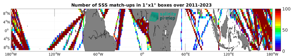
Figure 5: Number of SSS match-ups between TSG (LEGOS-DM) SSS and the SMAP SSS L4 OI v3 - Monthly (ESR) SSS product for the Equatorial Ocean 10N-10S Pi-MEP region over 1°×1° boxes and for the full satellite product period.
