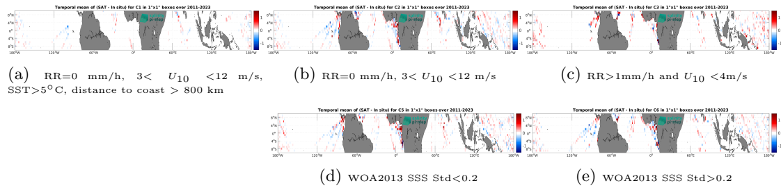
Figure 14: Temporal mean gridded over spatial boxes of size 1^\circ \times 1^\circ of \Delta SSS (SMAP SSS L4 OI v3 - Monthly (ESR) - TSG (LEGOS-DM)) for 5 different subdatasets corresponding to: RR=0 mm/h, 3 < U_{10} < 12 m/s, SST>5°C, distance to coast > 800 km (a), RR=0 mm/h, 3 < U_{10} < 12 m/s (b), RR>1mm/h and U_{10} < 4 m/s (c), WOA2013 SSS Std<0.2 (d), WOA2013 SSS Std>0.2 (e).
