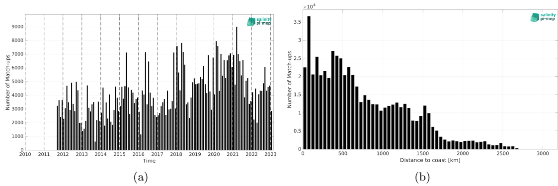
Figure 2: Number of match-ups between TSG (LEGOS-DM) and SMAP SSS L4 OI v3 - Monthly (ESR) SSS as a function of time (a) and as function of the distance to coast (b) over the Equatorial Ocean 10N-10S Pi-MEP region and for the full satellite product period.
