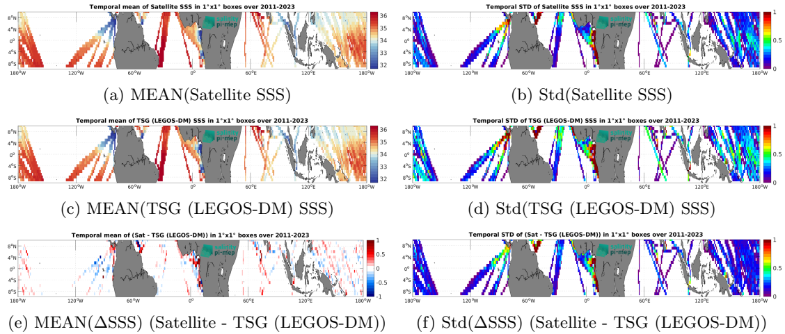
Figure 7: Temporal mean (left) and Std (right) of SSS from SMAP SSS L4 OI v3 - Monthly (ESR) (top), TSG (LEGOS-DM) (middle), and of \Delta SSS (Satellite - TSG (LEGOS-DM)). Only match-up pairs are used to generate these maps.
