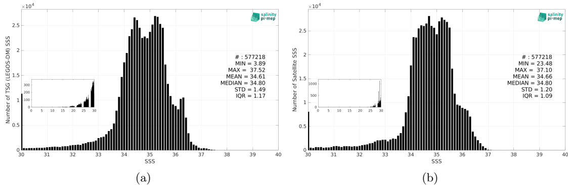
Figure 3: Histograms of SSS from TSG (LEGOS-DM) (a) and SMAP SSS L4 OI v3 - Monthly (ESR) (b) considering all match-up pairs per bins of 0.1 over the Equatorial Ocean 10N-10S Pi-MEP region and for the full satellite product period.
