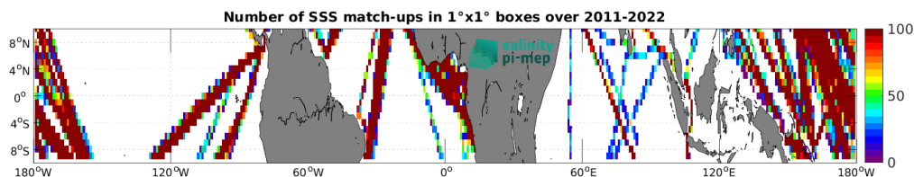
Figure 5: Number of SSS match-ups between TSG (LEGOS-DM) SSS and the SMAP SSS L4 OI v3 - Monthly (ESR) SSS product for the Equatorial Ocean 10N-10S Pi-MEP region over 1^\circ \times 1^\circ boxes and for the full satellite product period.
