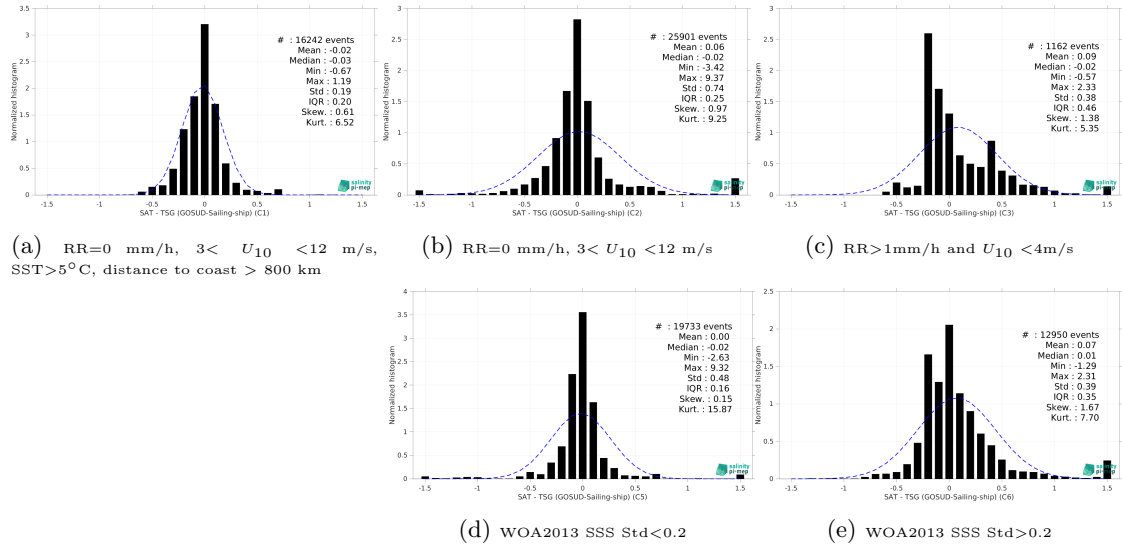
Figure 15: Normalized histogram of \Delta SSS (SMAP SSS L4 OI v3 - Monthly (ESR) - TSG (GOSUD-Sailing-ship)) for 5 different subdatasets corresponding to: RR=0 mm/h, 3 < U_{10} < 12 m/s, SST >5^\circ C, distance to coast > 800 km (a), RR=0 mm/h, 3 < U_{10} < 12 m/s (b), RR >1 mm/h and U_{10} < 4 m/s (c), WOA2013 SSS Std <0.2 (d), WOA2013 SSS Std >0.2 (e).
