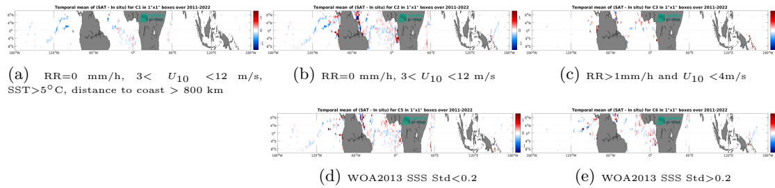
Figure 14: Temporal mean gridded over spatial boxes of size 1^\circ \times 1^\circ of \Delta SSS (SMAP SSS L4 OI v3 - Monthly (ESR) - TSG (GOSUD-Research-vessel)) for 5 different subdatasets corresponding to:RR=0 mm/h, 3 < U_{10} < 12 m/s, SST>5°C, distance to coast > 800 km (a), RR=0 mm/h, 3 < U_{10} < 12 m/s (b), RR>1mm/h and U_{10} < 4 m/s (c), WOA2013 SSS Std<0.2 (d), WOA2013 SSS Std>0.2 (e).
