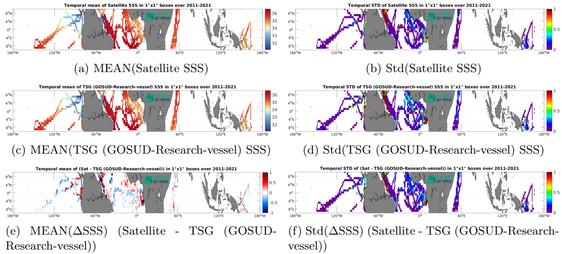
Figure 7: Temporal mean (left) and Std (right) of SSS from SMAP SSS L4 OI v3 - Monthly (ESR) (top), TSG (GOSUD-Research-vessel) (middle), and of \Delta SSS (Satellite - TSG (GOSUD-Research-vessel)). Only match-up pairs are used to generate these maps.
