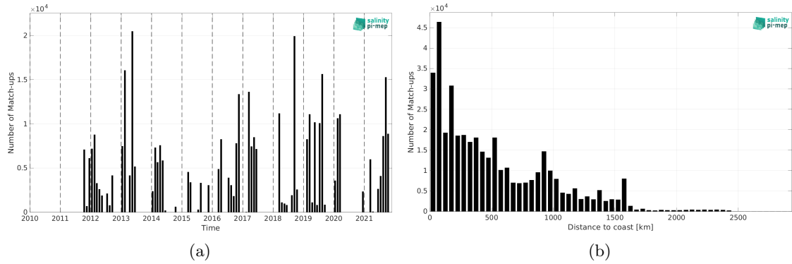
Figure 2: Number of match-ups between TSG (GOSUD-Research-vessel) and SMAP SSS L4 OI v3 - Monthly (ESR) SSS as a function of time (a) and as function of the distance to coast (b) over the Equatorial Ocean 10N-10S Pi-MEP region and for the full satellite product period.
