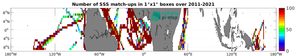
Figure 5: Number of SSS match-ups between TSG (GOSUD-Research-vessel) SSS and the SMAP SSS L4 OI v3 - Monthly (ESR) SSS product for the Equatorial Ocean 10N-10S Pi-MEP region over 1^\circ \times 1^\circ boxes and for the full satellite product period.
