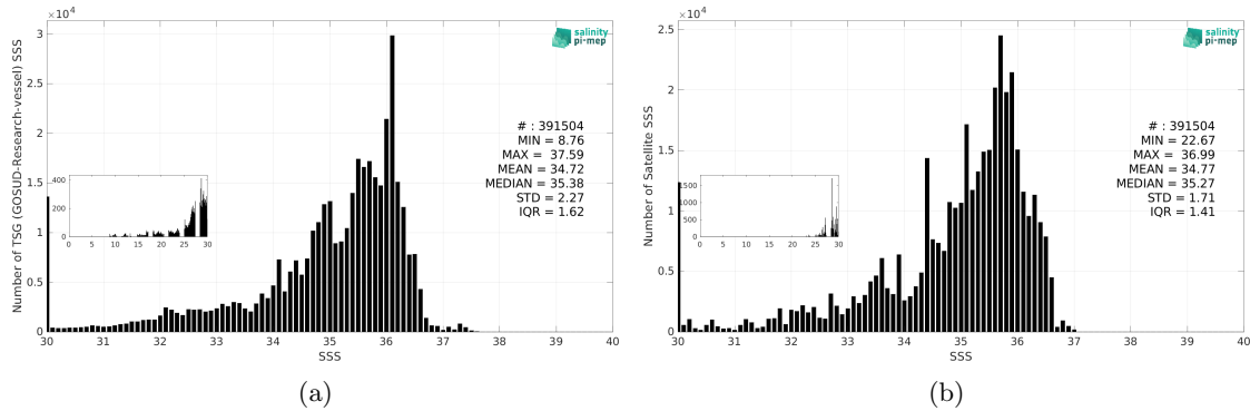
Figure 3: Histograms of SSS from TSG (GOSUD-Research-vessel) (a) and SMAP SSS L4 OI v3 - Monthly (ESR) (b) considering all match-up pairs per bins of 0.1 over the Equatorial Ocean 10N-10S Pi-MEP region and for the full satellite product period.
