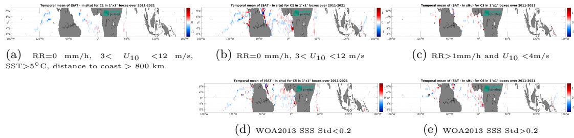
Figure 14: Temporal mean gridded over spatial boxes of size 1^\circ \times 1^\circ of \Delta\text{SSS} (SMAP SSS L4 OI v3 - Monthly (ESR) - TSG (GOSUD-Research-vessel)) for 5 different subdatasets corresponding to: RR=0 mm/h, 3 < U_{10} < 12 m/s, SST>5°C, distance to coast > 800 km (a), RR=0 mm/h, 3 < U_{10} < 12 m/s (b), RR>1mm/h and U_{10} < 4 m/s (c), WOA2013 SSS Std<0.2 (d), WOA2013 SSS Std>0.2 (e).
