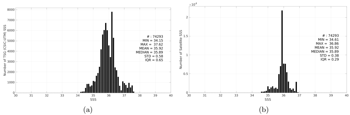
Figure 3: Histograms of SSS from TSG (CSIC-UTM) (a) and SMAP SSS L4 OI v3 - Monthly (ESR) (b) considering all match-up pairs per bins of 0.1 over the Equatorial Ocean 10N-10S Pi-MEP region and for the full satellite product period.
