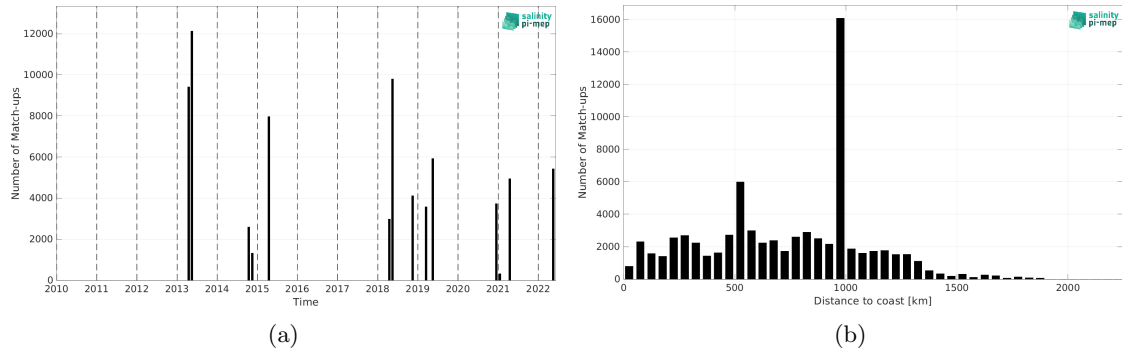
Figure 2: Number of match-ups between TSG (CSIC-UTM) and SMAP SSS L4 OI v3 - Monthly (ESR) SSS as a function of time (a) and as function of the distance to coast (b) over the Equatorial Ocean 10N-10S Pi-MEP region and for the full satellite product period.
