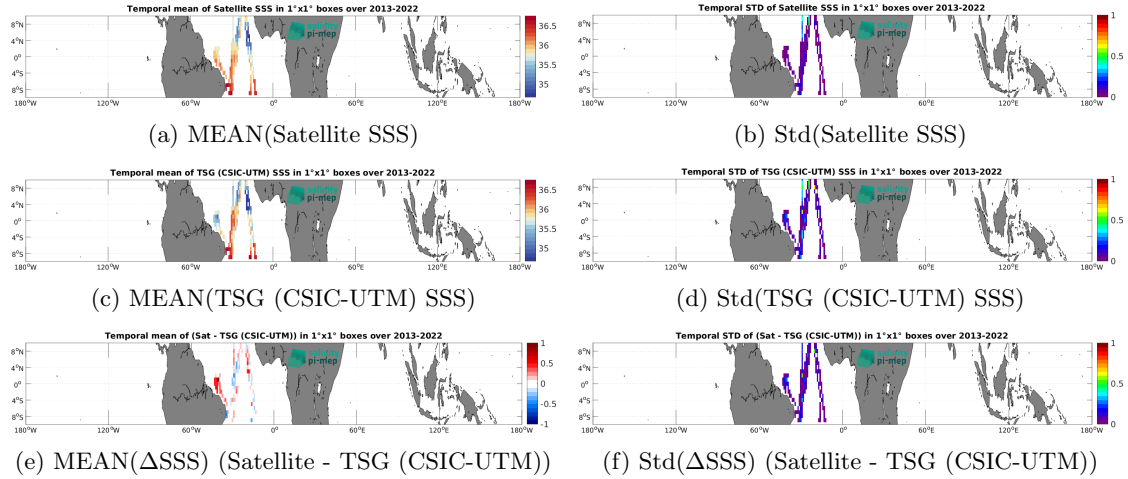
Figure 7: Temporal mean (left) and Std (right) of SSS from SMAP SSS L4 OI v3 - Monthly (ESR) (top), TSG (CSIC-UTM) (middle), and of \Delta SSS (Satellite - TSG (CSIC-UTM)). Only match-up pairs are used to generate these maps.
