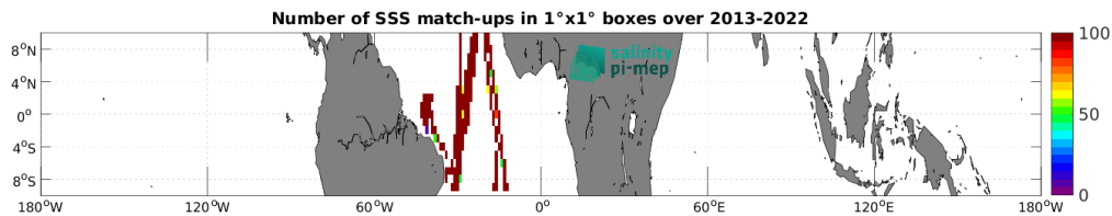
Figure 5: Number of SSS match-ups between TSG (CSIC-UTM) SSS and the SMAP SSS L4 OI v3 - Monthly (ESR) SSS product for the Equatorial Ocean 10N-10S Pi-MEP region over 1^\circ \times 1^\circ boxes and for the full satellite product period.
