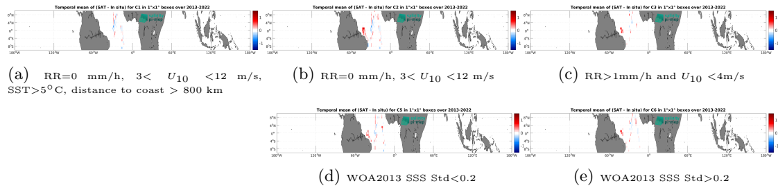
Figure 14: Temporal mean gridded over spatial boxes of size 1^\circ \times 1^\circ of \Delta SSS (SMAP SSS L4 OI v3 - Monthly (ESR) - TSG (CSIC-UTM)) for 5 different subdatasets corresponding to: RR=0 mm/h, 3 < U_{10} < 12 m/s, SST>5°C, distance to coast > 800 km (a), RR=0 mm/h, 3 < U_{10} < 12 m/s (b), RR>1mm/h and U_{10} < 4 m/s (c), WOA2013 SSS Std<0.2 (d), WOA2013 SSS Std>0.2 (e).
