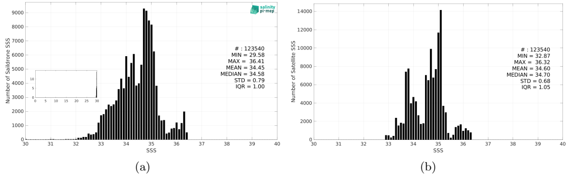
Figure 3: Histograms of SSS from Saildrone (a) and SMAP SSS L4 OI v3 - Monthly (ESR) (b) considering all match-up pairs per bins of 0.1 over the Equatorial Ocean 10N-10S Pi-MEP region and for the full satellite product period.
