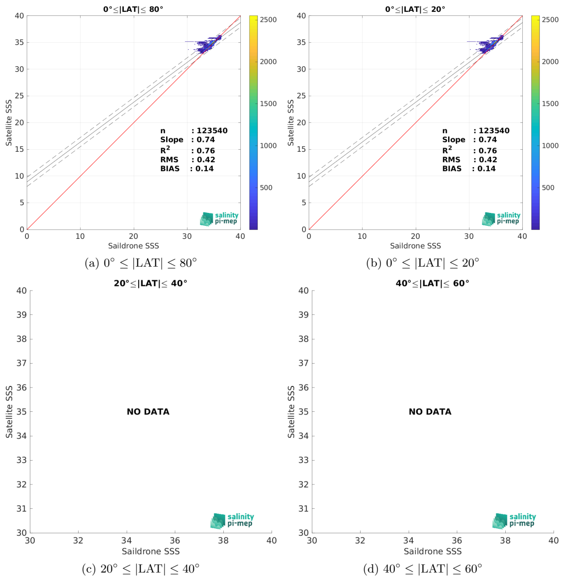
Figure 10: Contour maps of the concentration of SMAP SSS L4 OI v3 - Monthly (ESR) SSS (y-axis) versus Sairdrone SSS (x-axis) at match-up pairs for different latitude bands. For each plot, the red line shows x=y . The black thin and dashed lines indicate a linear fit through the data cloud and the \pm 95\% confidence levels, respectively. The number match-up pairs n , the slope and R^2 coefficient of the linear fit, the root mean square (RMS) and the mean bias between satellite and in situ data are indicated for each latitude band in each plots.
