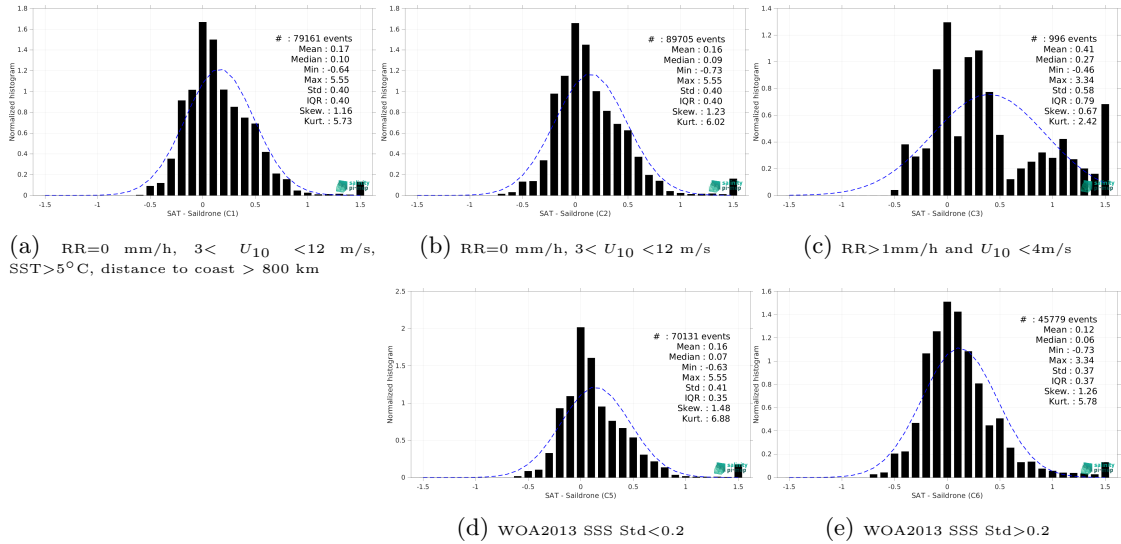
Figure 15: Normalized histogram of \Delta\text{SSS} (SMAP SSS L4 OI v3 - Monthly (ESR) - Saildrone) for 5 different subdatasets corresponding to: RR=0 mm/h, 3 < U_{10} < 12 m/s, SST>5°C, distance to coast > 800 km (a), RR=0 mm/h, 3 < U_{10} < 12 m/s (b), RR>1mm/h and U_{10} < 4 m/s (c), WOA2013 SSS Std<0.2 (d), WOA2013 SSS Std>0.2 (e).
