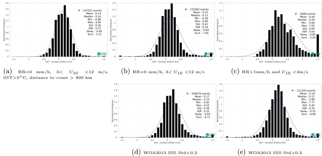
Figure 14: Normalized histogram of \Delta SSS (SMAP SSS L4 OI v3 - Monthly (ESR) - Surface drifters) for 5 different subdatasets corresponding to: RR=0 mm/h, 3 < U_{10} < 12 m/s, SST >5^\circ C, distance to coast > 800 km (a), RR=0 mm/h, 3 < U_{10} < 12 m/s (b), RR >1 mm/h and U_{10} < 4 m/s (c), WOA2013 SSS Std <0.2 (d), WOA2013 SSS Std >0.2 (e).
