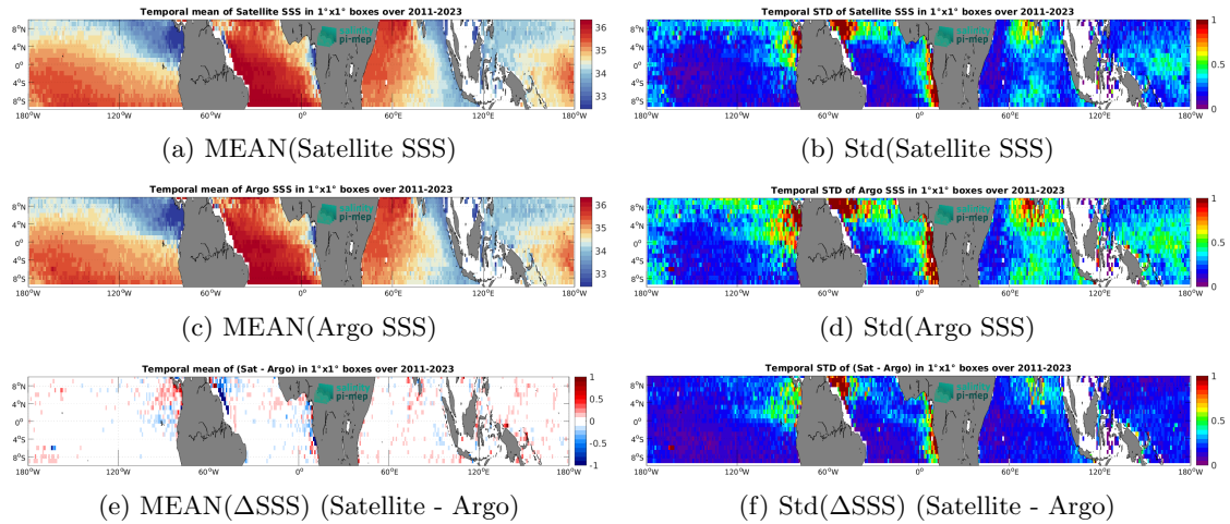
Figure 7: Temporal mean (left) and Std (right) of SSS from SMAP SSS L4 OI v3 - Monthly (ESR) (top), Argo (middle), and of \Delta SSS (Satellite - Argo). Only match-up pairs are used to generate these maps.
