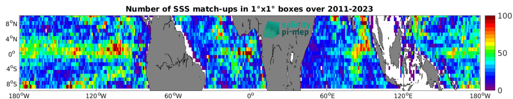
Figure 5: Number of SSS match-ups between Argo SSS and the SMAP SSS L4 OI v3 - Monthly (ESR) SSS product for the Equatorial Ocean 10N-10S Pi-MEP region over 1^\circ \times 1^\circ boxes and for the full satellite product period.
