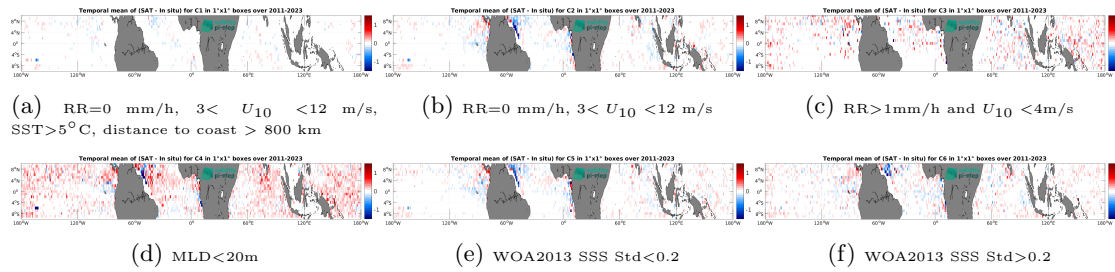
Figure 14: Temporal mean gridded over spatial boxes of size 1^\circ \times 1^\circ of \Delta SSS (SMAP SSS L4 OI v3 - Monthly (ESR) - Argo) for 6 different subdatasets corresponding to:RR=0 mm/h, 3 < U_{10} < 12 m/s, SST >5^\circ\text{C} , distance to coast > 800 km (a), RR=0 mm/h, 3 < U_{10} < 12 m/s (b), RR >1 mm/h and U_{10} < 4 m/s (c),MLD <20 m (d),WOA2013 SSS Std <0.2 (e),WOA2013 SSS Std >0.2 (f).
