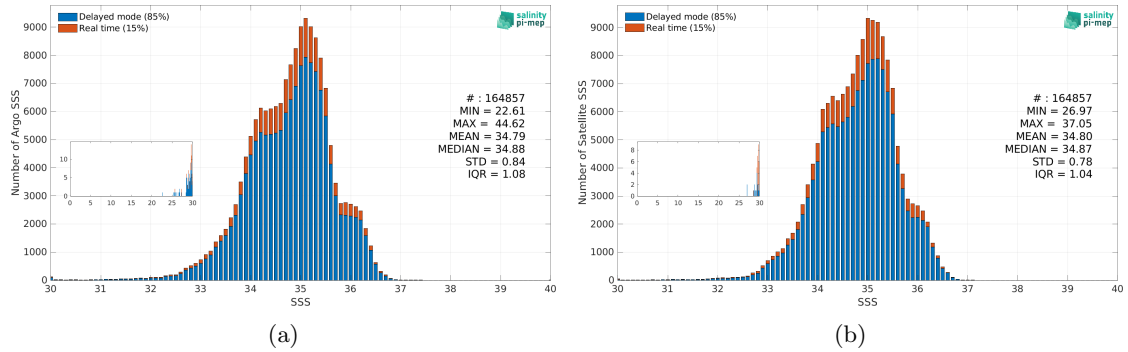
Figure 3: Histograms of SSS from Argo (a) and SMAP SSS L4 OI v3 - Monthly (ESR) (b) considering all match-up pairs per bins of 0.1 over the Equatorial Ocean 10N-10S Pi-MEP region and for the full satellite product period.
