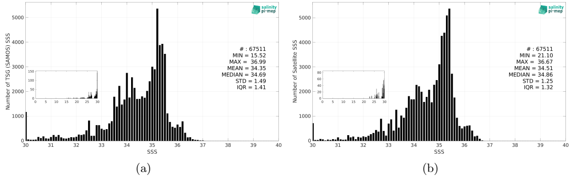
Figure 3: Histograms of SSS from TSG (SAMOS) (a) and SMAP SSS L4 OI v3 - Daily (ESR) (b) considering all match-up pairs per bins of 0.1 over the Equatorial Ocean 10N-10S Pi-MEP region and for the full satellite product period.
