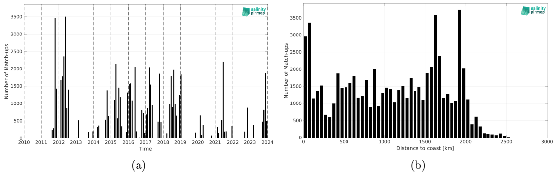
Figure 2: Number of match-ups between TSG (SAMOS) and SMAP SSS L4 OI v3 - Daily (ESR) SSS as a function of time (a) and as function of the distance to coast (b) over the Equatorial Ocean 10N-10S Pi-MEP region and for the full satellite product period.
