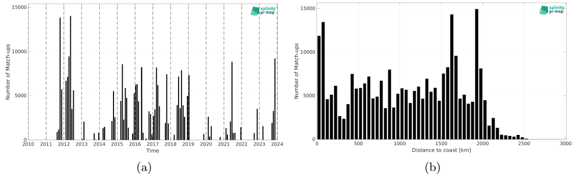
Figure 2: Number of match-ups between TSG (SAMOS) and SMAP SSS L4 OI v3 - Daily (ESR) SSS as a function of time (a) and as function of the distance to coast (b) over the Equatorial Ocean 10N-10S Pi-MEP region and for the full satellite product period.
