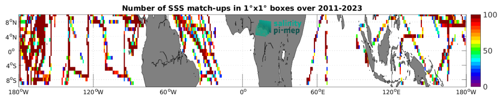
Figure 5: Number of SSS match-ups between TSG (SAMOS) SSS and the SMAP SSS L4 OI v3 - Daily (ESR) SSS product for the Equatorial Ocean 10N-10S Pi-MEP region over 1^\circ \times 1^\circ boxes and for the full satellite product period.
