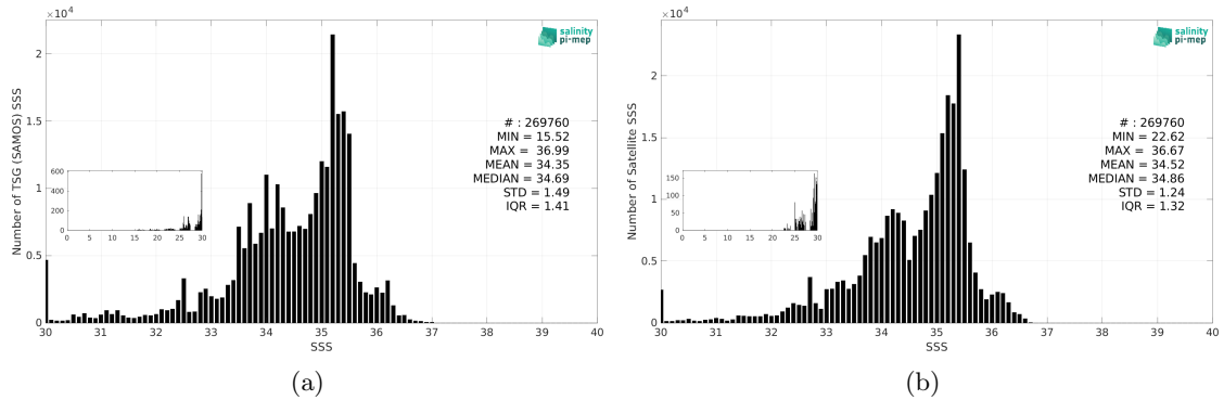
Figure 3: Histograms of SSS from TSG (SAMOS) (a) and SMAP SSS L4 OI v3 - Daily (ESR) (b) considering all match-up pairs per bins of 0.1 over the Equatorial Ocean 10N-10S Pi-MEP region and for the full satellite product period.
