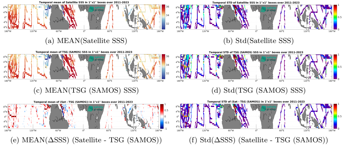
Figure 7: Temporal mean (left) and Std (right) of SSS from SMAP SSS L4 OI v3 - Daily (ESR) (top), TSG (SAMOS) (middle), and of \Delta SSS (Satellite - TSG (SAMOS)). Only match-up pairs are used to generate these maps.
