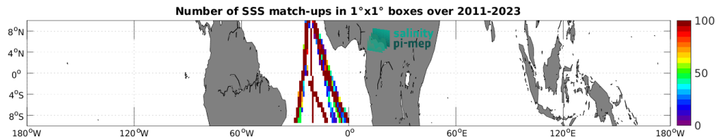
Figure 5: Number of SSS match-ups between TSG (Polarstern) SSS and the SMAP SSS L4 OI v3 - Daily (ESR) SSS product for the Equatorial Ocean 10N-10S Pi-MEP region over 1^\circ \times 1^\circ boxes and for the full satellite product period.
