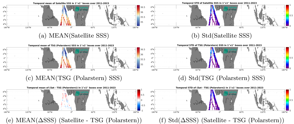
Figure 7: Temporal mean (left) and Std (right) of SSS from SMAP SSS L4 OI v3 - Daily (ESR) (top), TSG (Polarstern) (middle), and of \Delta SSS (Satellite - TSG (Polarstern)). Only match-up pairs are used to generate these maps.
