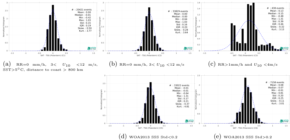
Figure 15: Normalized histogram of \Delta\text{SSS} (SMAP SSS L4 OI v3 - Daily (ESR) - TSG (Polarstern)) for 5 different subdatasets corresponding to: RR=0 mm/h, 3 < U_{10} < 12 m/s, SST>5°C, distance to coast > 800 km (a), RR=0 mm/h, 3 < U_{10} < 12 m/s (b), RR>1mm/h and U_{10} < 4 m/s (c), WOA2013 SSS Std<0.2 (d), WOA2013 SSS Std>0.2 (e).
