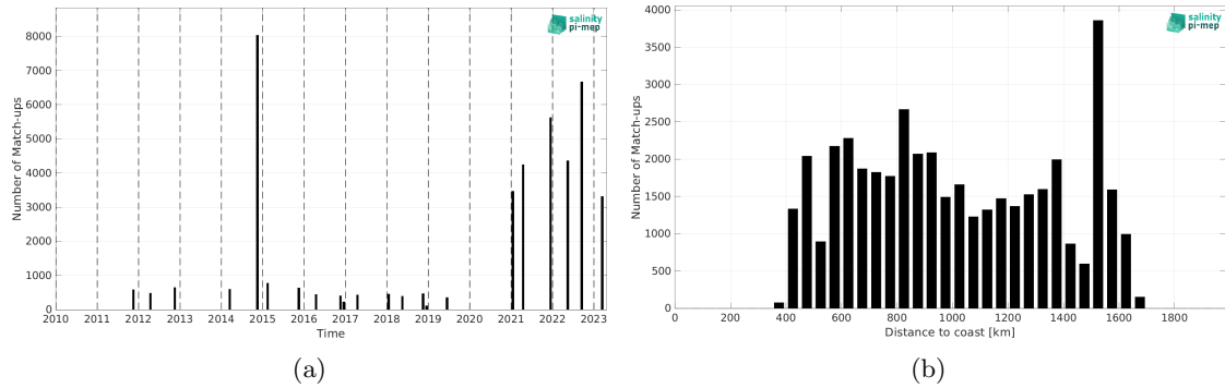
Figure 2: Number of match-ups between TSG (Polarstern) and SMAP SSS L4 OI v3 - Daily (ESR) SSS as a function of time (a) and as function of the distance to coast (b) over the Equatorial Ocean 10N-10S Pi-MEP region and for the full satellite product period.
