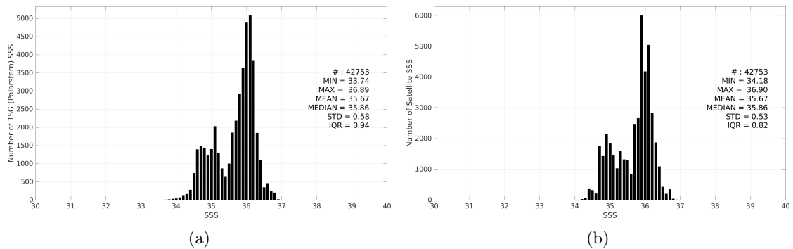
Figure 3: Histograms of SSS from TSG (Polarstern) (a) and SMAP SSS L4 OI v3 - Daily (ESR) (b) considering all match-up pairs per bins of 0.1 over the Equatorial Ocean 10N-10S Pi-MEP region and for the full satellite product period.
