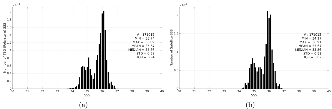
Figure 3: Histograms of SSS from TSG (Polarstern) (a) and SMAP SSS L4 OI v3 - Daily (ESR) (b) considering all match-up pairs per bins of 0.1 over the Equatorial Ocean 10N-10S Pi-MEP region and for the full satellite product period.
