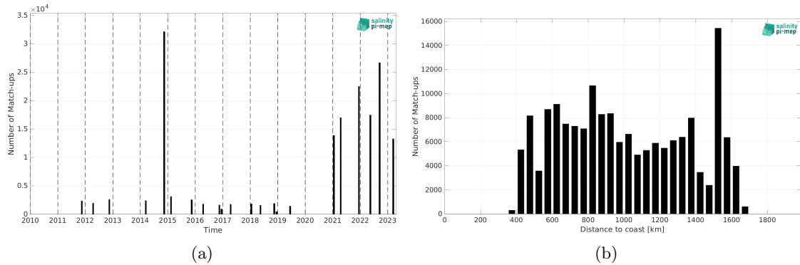
Figure 2: Number of match-ups between TSG (Polarstern) and SMAP SSS L4 OI v3 - Daily (ESR) SSS as a function of time (a) and as function of the distance to coast (b) over the Equatorial Ocean 10N-10S Pi-MEP region and for the full satellite product period.
