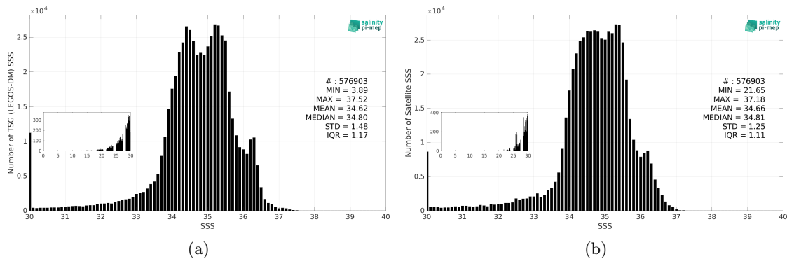
Figure 3: Histograms of SSS from TSG (LEGOS-DM) (a) and SMAP SSS L4 OI v3 - Daily (ESR) (b) considering all match-up pairs per bins of 0.1 over the Equatorial Ocean 10N-10S Pi-MEP region and for the full satellite product period.
