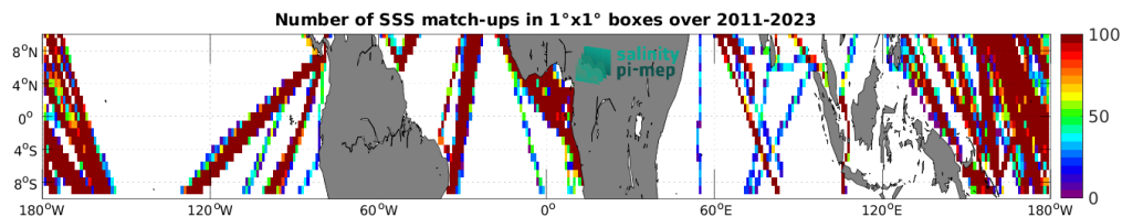
Figure 5: Number of SSS match-ups between TSG (LEGOS-DM) SSS and the SMAP SSS L4 OI v3 - Daily (ESR) SSS product for the Equatorial Ocean 10N-10S Pi-MEP region over 1^\circ \times 1^\circ boxes and for the full satellite product period.
