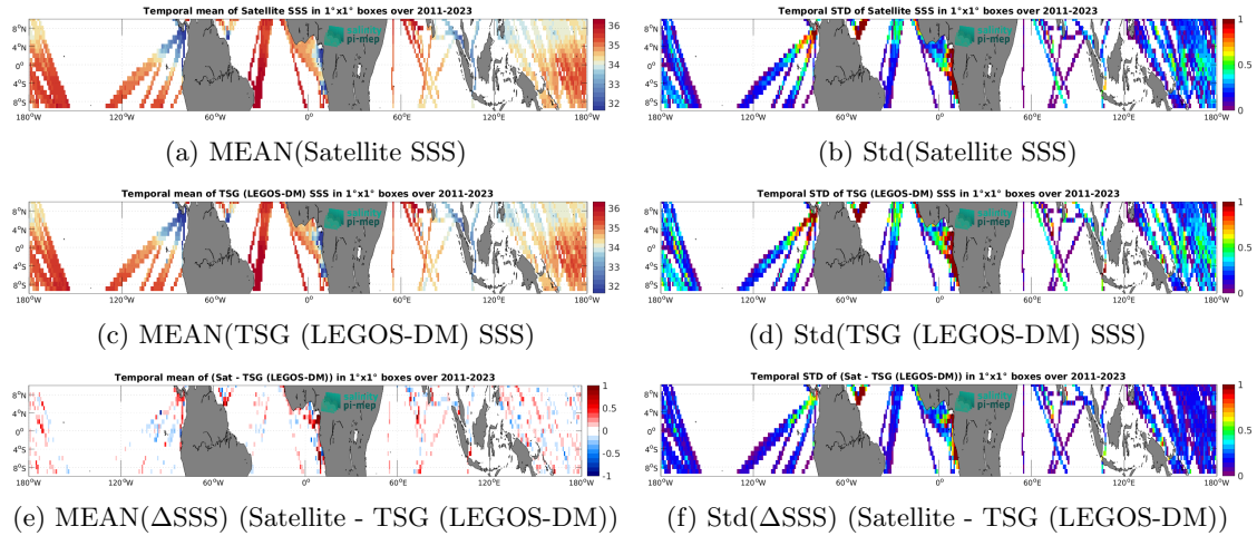
Figure 7: Temporal mean (left) and Std (right) of SSS from SMAP SSS L4 OI v3 - Daily (ESR) (top), TSG (LEGOS-DM) (middle), and of \Delta SSS (Satellite - TSG (LEGOS-DM)). Only match-up pairs are used to generate these maps.
