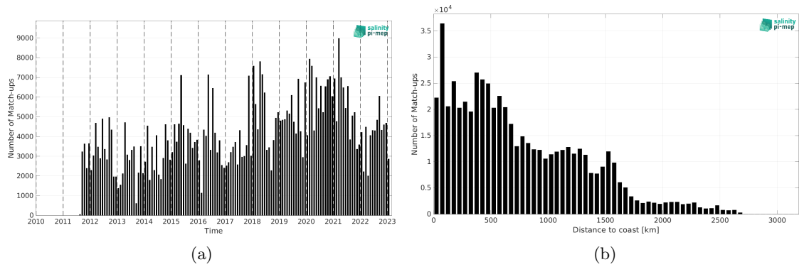
Figure 2: Number of match-ups between TSG (LEGOS-DM) and SMAP SSS L4 OI v3 - Daily (ESR) SSS as a function of time (a) and as function of the distance to coast (b) over the Equatorial Ocean 10N-10S Pi-MEP region and for the full satellite product period.
