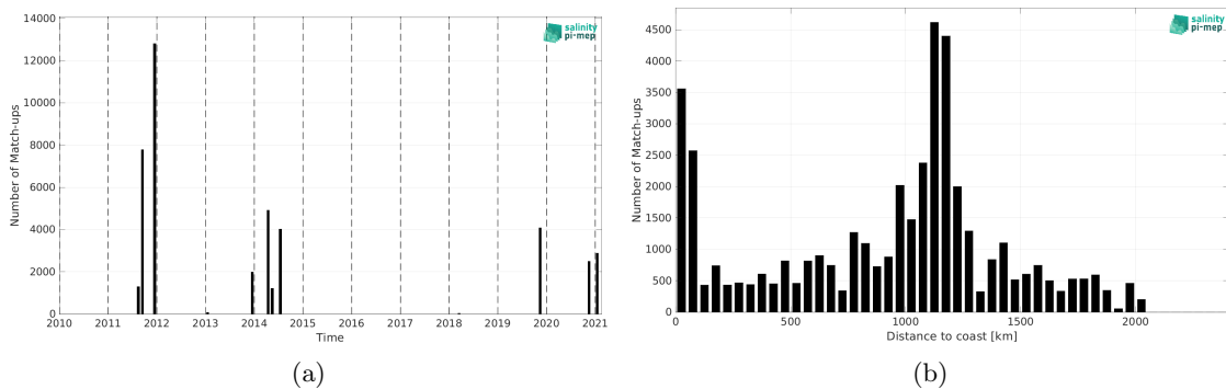
Figure 2: Number of match-ups between TSG (GOSUD-Sailing-ship) and SMAP SSS L4 OI v3 - Daily (ESR) SSS as a function of time (a) and as function of the distance to coast (b) over the Equatorial Ocean 10N-10S Pi-MEP region and for the full satellite product period.
