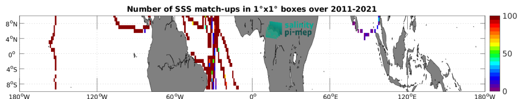
Figure 5: Number of SSS match-ups between TSG (GOSUD-Sailing-ship) SSS and the SMAP SSS L4 OI v3 - Daily (ESR) SSS product for the Equatorial Ocean 10N-10S Pi-MEP region over 1^\circ \times 1^\circ boxes and for the full satellite product period.
