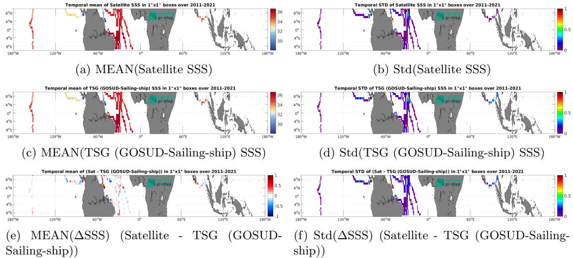
Figure 7: Temporal mean (left) and Std (right) of SSS from SMAP SSS L4 OI v3 - Daily (ESR) (top), TSG (GOSUD-Sailing-ship) (middle), and of \Delta SSS (Satellite - TSG (GOSUD-Sailing-ship)). Only match-up pairs are used to generate these maps.
