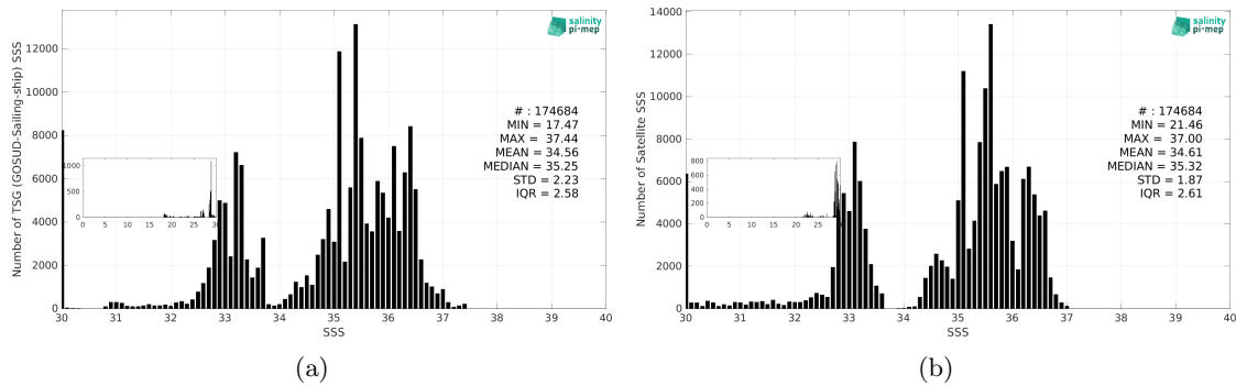
Figure 3: Histograms of SSS from TSG (GOSUD-Sailing-ship) (a) and SMAP SSS L4 OI v3 - Daily (ESR) (b) considering all match-up pairs per bins of 0.1 over the Equatorial Ocean 10N-10S Pi-MEP region and for the full satellite product period.
