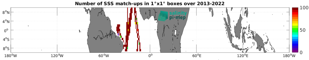
Figure 5: Number of SSS match-ups between TSG (CSIC-UTM) SSS and the SMAP SSS L4 OI v3 - Daily (ESR) SSS product for the Equatorial Ocean 10N-10S Pi-MEP region over 1^\circ \times 1^\circ boxes and for the full satellite product period.
