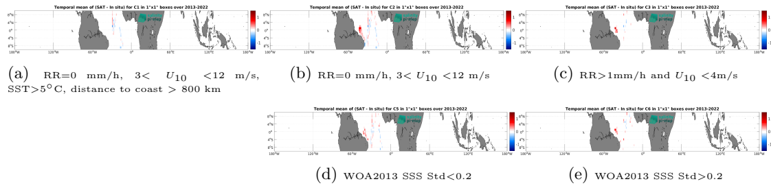
Figure 14: Temporal mean gridded over spatial boxes of size 1^\circ \times 1^\circ of \Delta\text{SSS} (SMAP SSS L4 OI v3 - Daily (ESR) - TSG (CSIC-UTM)) for 5 different subdatasets corresponding to: RR=0 mm/h, 3 < U_{10} < 12 m/s, SST>5°C, distance to coast > 800 km (a), RR=0 mm/h, 3 < U_{10} < 12 m/s (b), RR>1mm/h and U_{10} < 4 m/s (c), WOA2013 SSS Std<0.2 (d), WOA2013 SSS Std>0.2 (e).
