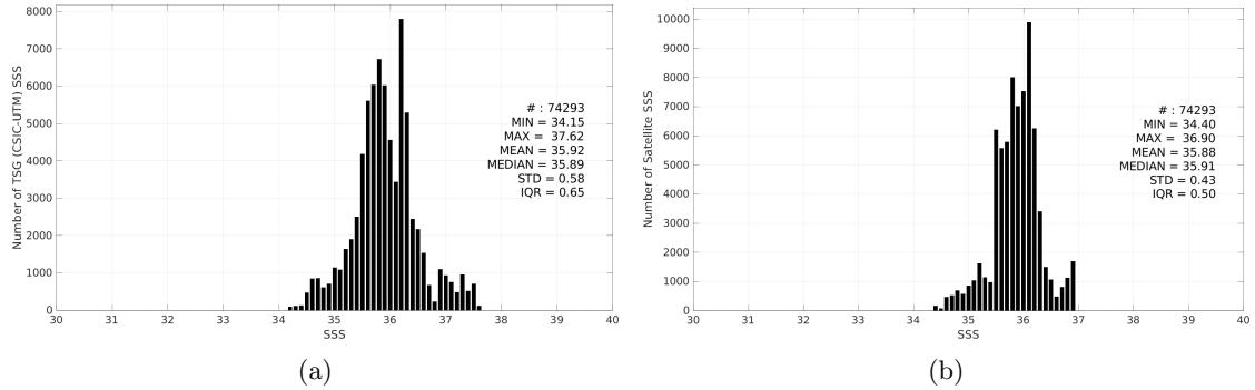
Figure 3: Histograms of SSS from TSG (CSIC-UTM) (a) and SMAP SSS L4 OI v3 - Daily (ESR) (b) considering all match-up pairs per bins of 0.1 over the Equatorial Ocean 10N-10S Pi-MEP region and for the full satellite product period.
