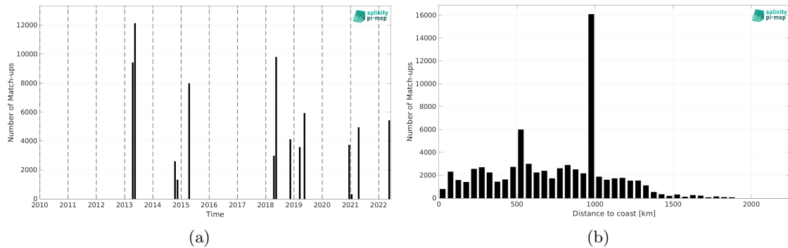
Figure 2: Number of match-ups between TSG (CSIC-UTM) and SMAP SSS L4 OI v3 - Daily (ESR) SSS as a function of time (a) and as function of the distance to coast (b) over the Equatorial Ocean 10N-10S Pi-MEP region and for the full satellite product period.
