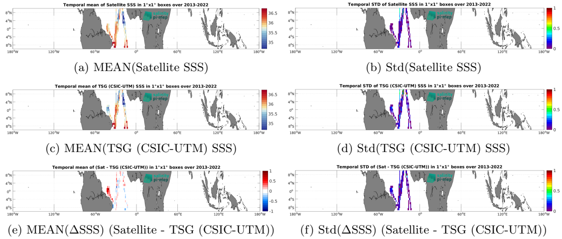
Figure 7: Temporal mean (left) and Std (right) of SSS from SMAP SSS L4 OI v3 - Daily (ESR) (top), TSG (CSIC-UTM) (middle), and of \Delta SSS (Satellite - TSG (CSIC-UTM)). Only match-up pairs are used to generate these maps.
