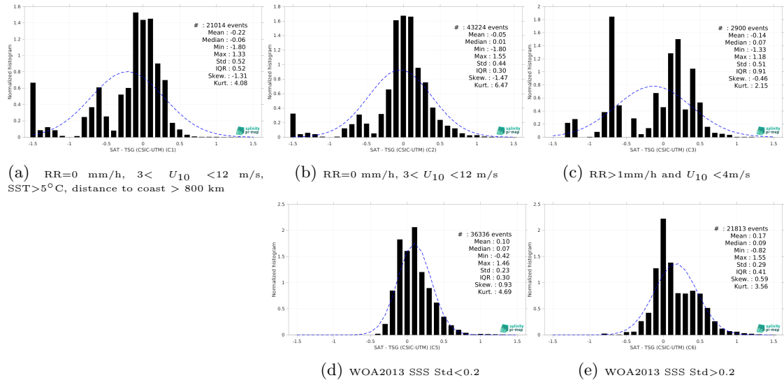
Figure 15: Normalized histogram of \Delta\text{SSS} (SMAP SSS L4 OI v3 - Daily (ESR) - TSG (CSIC-UTM)) for 5 different subdatasets corresponding to: RR=0 mm/h, 3 < U_{10} < 12 m/s, SST>5°C, distance to coast > 800 km (a), RR=0 mm/h, 3 < U_{10} < 12 m/s (b), RR>1mm/h and U_{10} < 4 m/s (c), WOA2013 SSS Std<0.2 (d), WOA2013 SSS Std>0.2 (e).
