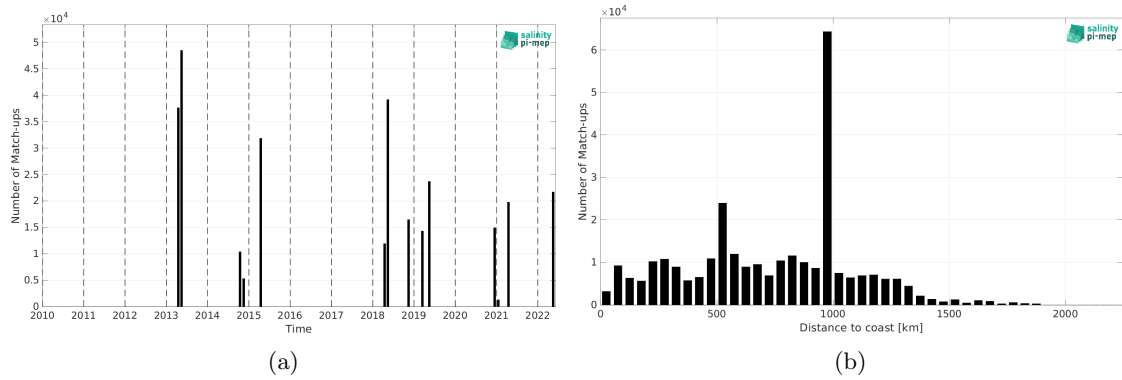
Figure 2: Number of match-ups between TSG (CSIC-UTM) and SMAP SSS L4 OI v3 - Daily (ESR) SSS as a function of time (a) and as function of the distance to coast (b) over the Equatorial Ocean 10N-10S Pi-MEP region and for the full satellite product period.
