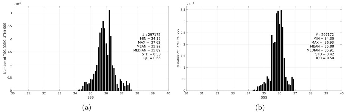
Figure 3: Histograms of SSS from TSG (CSIC-UTM) (a) and SMAP SSS L4 OI v3 - Daily (ESR) (b) considering all match-up pairs per bins of 0.1 over the Equatorial Ocean 10N-10S Pi-MEP region and for the full satellite product period.
