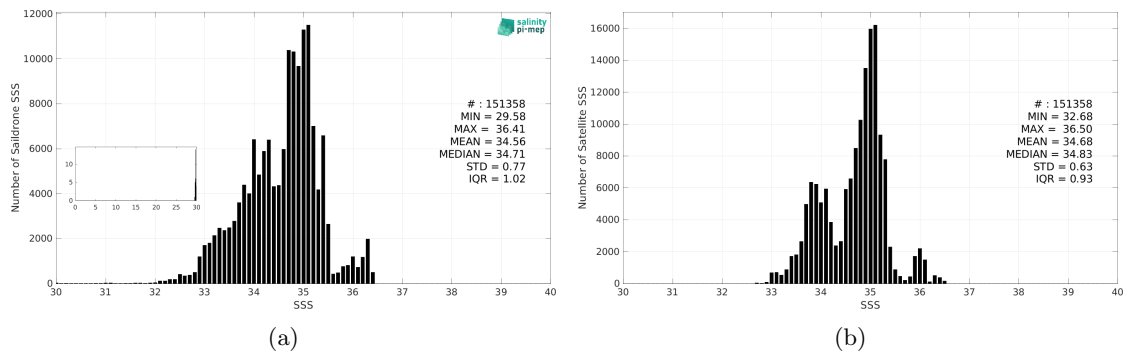
Figure 3: Histograms of SSS from Saildrone (a) and SMAP SSS L4 OI v3 - Daily (ESR) (b) considering all match-up pairs per bins of 0.1 over the Equatorial Ocean 10N-10S Pi-MEP region and for the full satellite product period.
