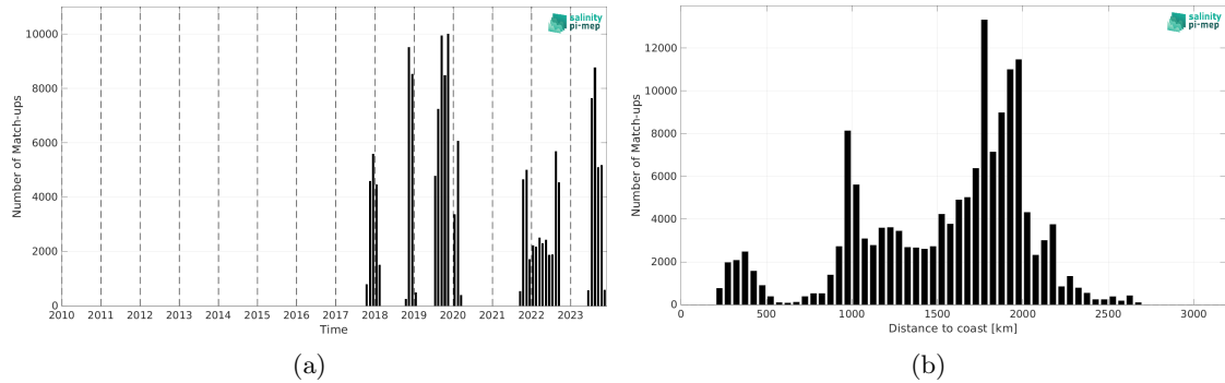
Figure 2: Number of match-ups between Saildrone and SMAP SSS L4 OI v3 - Daily (ESR) SSS as a function of time (a) and as function of the distance to coast (b) over the Equatorial Ocean 10N-10S Pi-MEP region and for the full satellite product period.
