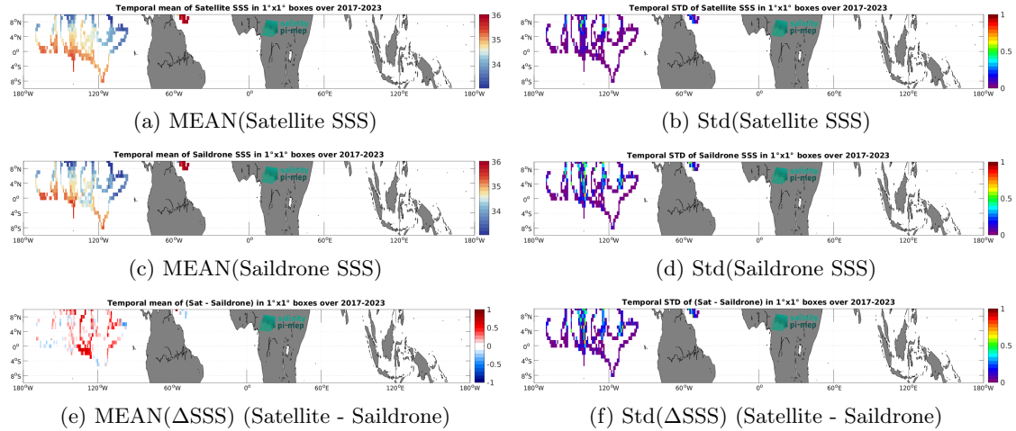
Figure 7: Temporal mean (left) and Std (right) of SSS from SMAP SSS L4 OI v3 - Daily (ESR) (top), Saildrone (middle), and of \Delta SSS (Satellite - Saildrone). Only match-up pairs are used to generate these maps.
