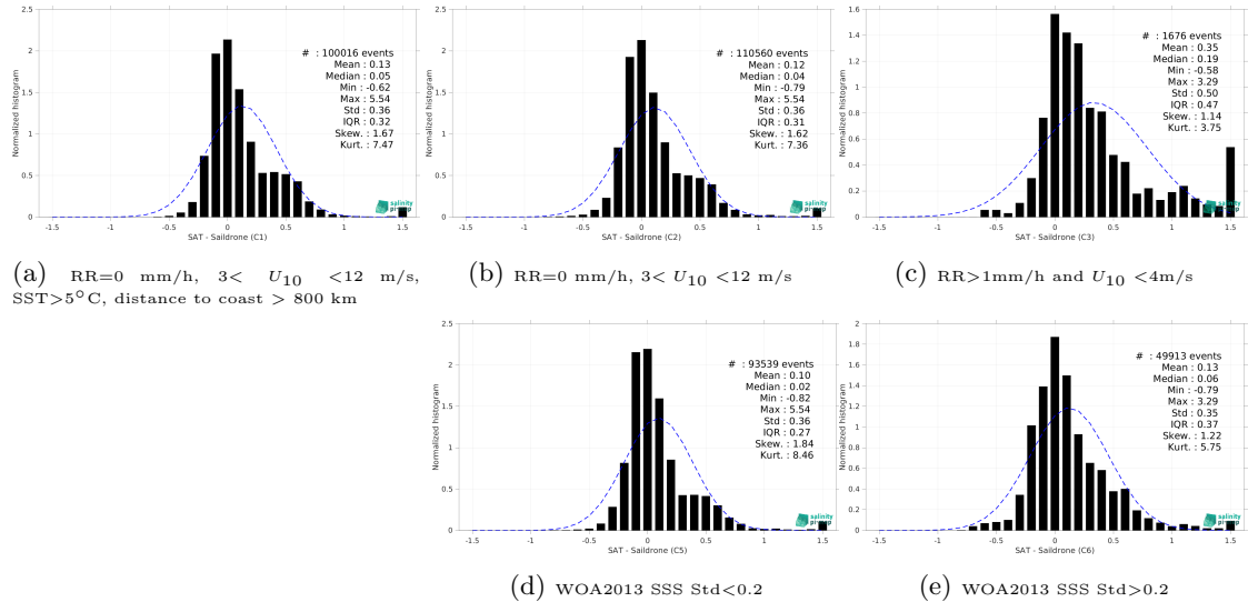
Figure 15: Normalized histogram of \Delta SSS (SMAP SSS L4 OI v3 - Daily (ESR) - Saildrone) for 5 different subdatasets corresponding to: RR=0 mm/h, 3 < U_{10} < 12 m/s, SST>5°C, distance to coast > 800 km (a), RR=0 mm/h, 3 < U_{10} < 12 m/s (b), RR>1mm/h and U_{10} < 4 m/s (c), WOA2013 SSS Std<0.2 (d), WOA2013 SSS Std>0.2 (e).
