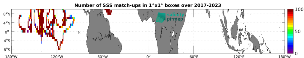
Figure 5: Number of SSS match-ups between Saildrone SSS and the SMAP SSS L4 OI v3 - Daily (ESR) SSS product for the Equatorial Ocean 10N-10S Pi-MEP region over 1^\circ \times 1^\circ boxes and for the full satellite product period.
