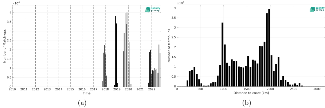
Figure 2: Number of match-ups between Saildrone and SMAP SSS L4 OI v3 - Daily (ESR) SSS as a function of time (a) and as function of the distance to coast (b) over the Equatorial Ocean 10N-10S Pi-MEP region and for the full satellite product period.
