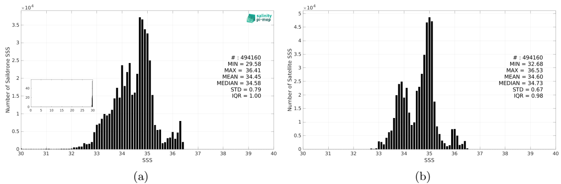
Figure 3: Histograms of SSS from Saildrone (a) and SMAP SSS L4 OI v3 - Daily (ESR) (b) considering all match-up pairs per bins of 0.1 over the Equatorial Ocean 10N-10S Pi-MEP region and for the full satellite product period.
