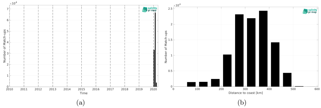
Figure 2: Number of match-ups between EUREC4A and SMAP SSS L4 OI v3 - Daily (ESR) SSS as a function of time (a) and as function of the distance to coast (b) over the Equatorial Ocean 10N-10S Pi-MEP region and for the full satellite product period.
