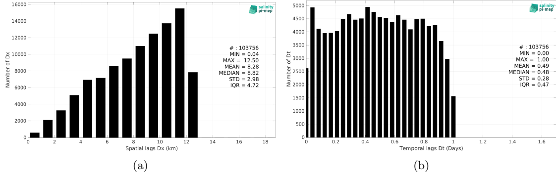
Figure 6: Histograms of the spatial (a) and temporal (b) lags between the location/time of the EUREC4A measurement and the date of the corresponding SMAP SSS L4 OI v3 - Daily (ESR) SSS pixel.
