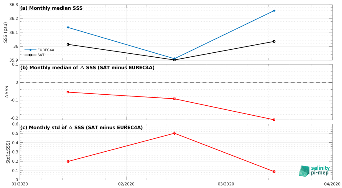
Figure 8: Time series of the monthly median SSS (top), median of \Delta SSS (Satellite - EUREC4A) and Std of \Delta SSS (Satellite - EUREC4A) over the Equatorial Ocean 10N-10S Pi-MEP region considering all match-ups collected by the Pi-MEP.
