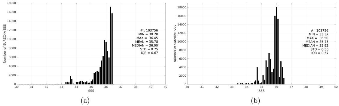
Figure 3: Histograms of SSS from EUREC4A (a) and SMAP SSS L4 OI v3 - Daily (ESR) (b) considering all match-up pairs per bins of 0.1 over the Equatorial Ocean 10N-10S Pi-MEP region and for the full satellite product period.
