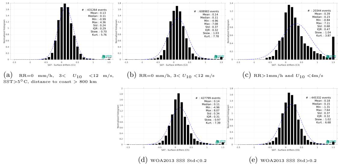
Figure 14: Normalized histogram of \Delta SSS (SMAP SSS L4 OI v3 - Daily (ESR) - Surface drifters) for 5 different subdatasets corresponding to: RR=0 mm/h, 3 < U_{10} < 12 m/s, SST >5^\circ C, distance to coast > 800 km (a), RR=0 mm/h, 3 < U_{10} < 12 m/s (b), RR >1 mm/h and U_{10} < 4 m/s (c), WOA2013 SSS Std <0.2 (d), WOA2013 SSS Std >0.2 (e).
