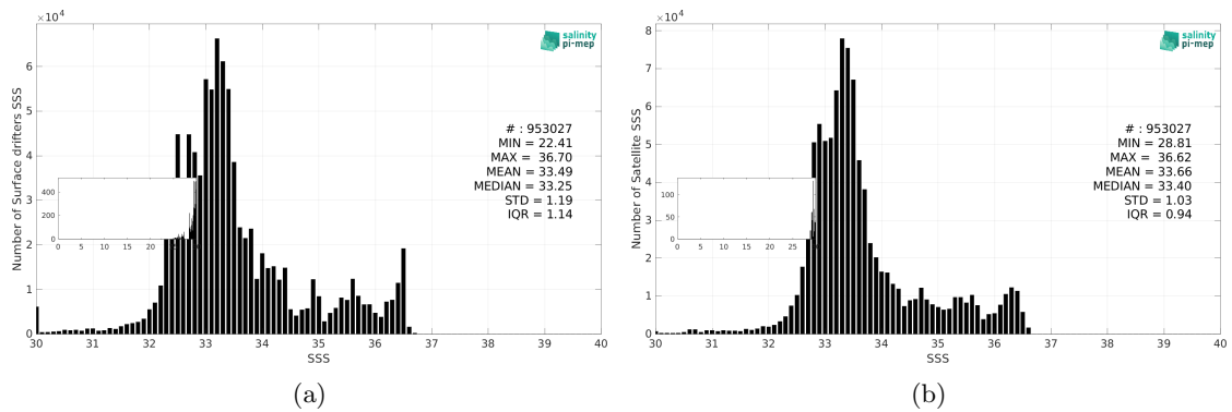
Figure 3: Histograms of SSS from Surface drifters (a) and SMAP SSS L4 OI v3 - Daily (ESR) (b) considering all match-up pairs per bins of 0.1 over the Equatorial Ocean 10N-10S Pi-MEP region and for the full satellite product period.
