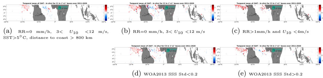
Figure 13: Temporal mean gridded over spatial boxes of size 1^\circ \times 1^\circ of \Delta SSS (SMAP SSS L4 OI v3 - Daily (ESR) - Surface drifters) for 5 different subdatasets corresponding to:RR=0 mm/h, 3 < U_{10} < 12 m/s, SST >5^\circ C, distance to coast > 800 km (a), RR=0 mm/h, 3 < U_{10} < 12 m/s (b), RR >1 mm/h and U_{10} < 4 m/s (c), WOA2013 SSS Std <0.2 (d), WOA2013 SSS Std >0.2 (e).
