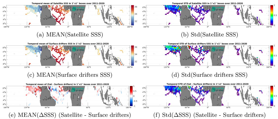
Figure 6: Temporal mean (left) and Std (right) of SSS from SMAP SSS L4 OI v3 - Daily (ESR) (top), Surface drifters (middle), and of \Delta SSS (Satellite - Surface drifters). Only match-up pairs are used to generate these maps.
