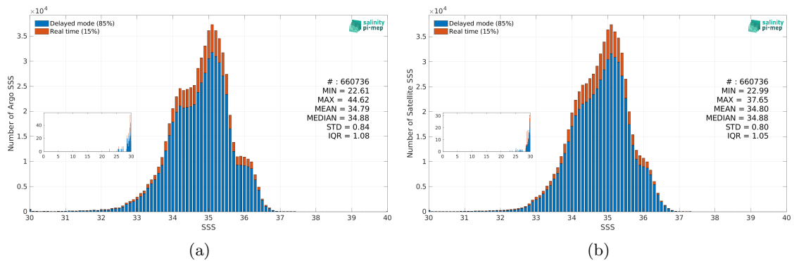
Figure 3: Histograms of SSS from Argo (a) and SMAP SSS L4 OI v3 - Daily (ESR) (b) considering all match-up pairs per bins of 0.1 over the Equatorial Ocean 10N-10S Pi-MEP region and for the full satellite product period.
