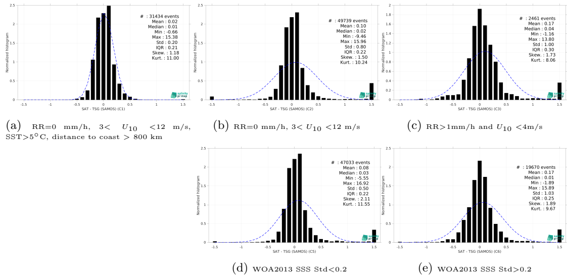
Figure 13: Normalized histogram of \Delta SSS (SMAP SSS L4 OI v2 - 7 Days (ESR) - TSG (SAMOS)) for 5 different subdatasets corresponding to: RR=0 mm/h, 3 < U_{10} < 12 m/s, SST >5^\circ C, distance to coast > 800 km (a), RR=0 mm/h, 3 < U_{10} < 12 m/s (b), RR >1 mm/h and U_{10} < 4 m/s (c), WOA2013 SSS Std <0.2 (d), WOA2013 SSS Std >0.2 (e).
