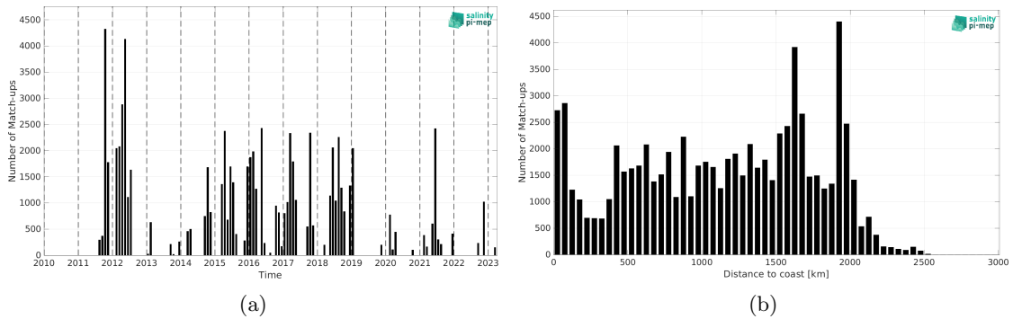
Figure 1: Number of match-ups between TSG (SAMOS) and SMAP SSS L4 OI v2 - 7 Days (ESR) SSS as a function of time (a) and as function of the distance to coast (b) over the Equatorial Ocean 10N-10S Pi-MEP region and for the full satellite product period.
