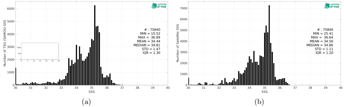
Figure 2: Histograms of SSS from TSG (SAMOS) (a) and SMAP SSS L4 OI v2 - 7 Days (ESR) (b) considering all match-up pairs per bins of 0.1 over the Equatorial Ocean 10N-10S Pi-MEP region and for the full satellite product period.
