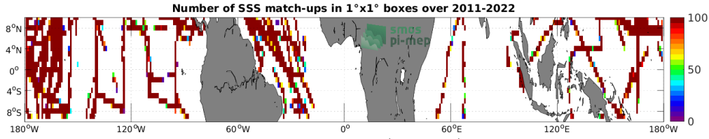
Figure 4: Number of SSS match-ups between TSG (SAMOS) SSS and the SMAP SSS L4 OI v2 - 7 Days (ESR) SSS product for the Equatorial Ocean 10N-10S Pi-MEP region over 1^\circ \times 1^\circ boxes and for the full satellite product period.
