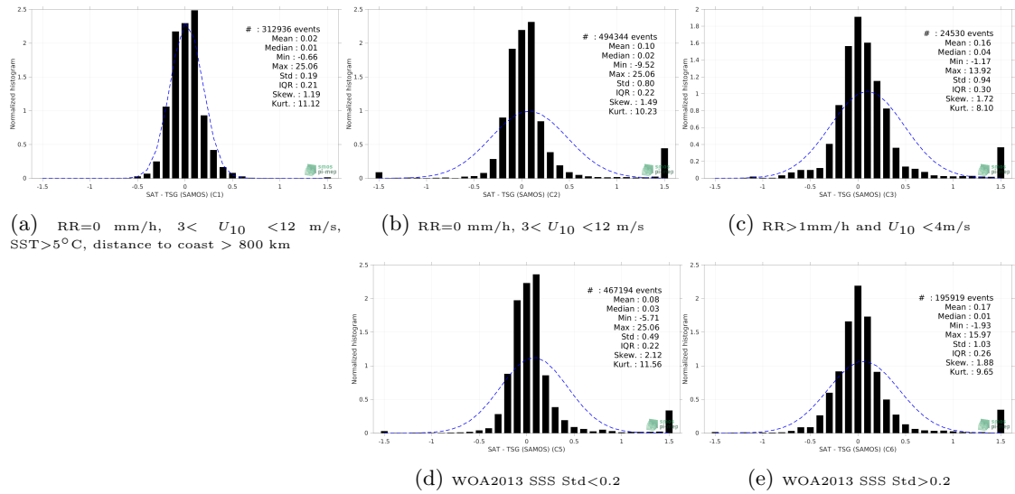
Figure 13: Normalized histogram of \Delta SSS (SMAP SSS L4 OI v2 - 7 Days (ESR) - TSG (SAMOS)) for 5 different subdatasets corresponding to: RR=0 mm/h, 3 < U_{10} < 12 m/s, SST > 5^\circ C , distance to coast > 800 km (a), RR=0 mm/h, 3 < U_{10} < 12 m/s (b), RR>1mm/h and U_{10} < 4 m/s (c), WOA2013 SSS Std<0.2 (d), WOA2013 SSS Std>0.2 (e).
