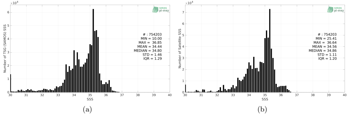
Figure 2: Histograms of SSS from TSG (SAMOS) (a) and SMAP SSS L4 OI v2 - 7 Days (ESR) (b) considering all match-up pairs per bins of 0.1 over the Equatorial Ocean 10N-10S Pi-MEP region and for the full satellite product period.
