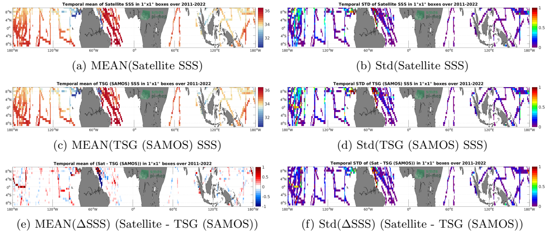
Figure 6: Temporal mean (left) and Std (right) of SSS from SMAP SSS L4 OI v2 - 7 Days (ESR) (top), TSG (SAMOS) (middle), and of \Delta SSS (Satellite - TSG (SAMOS)). Only match-up pairs are used to generate these maps.
