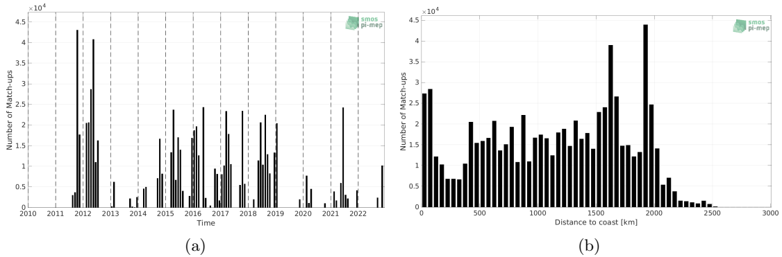
Figure 1: Number of match-ups between TSG (SAMOS) and SMAP SSS L4 OI v2 - 7 Days (ESR) SSS as a function of time (a) and as function of the distance to coast (b) over the Equatorial Ocean 10N-10S Pi-MEP region and for the full satellite product period.
