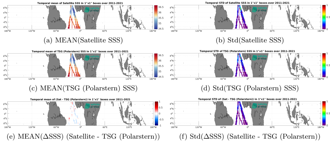
Figure 6: Temporal mean (left) and Std (right) of SSS from SMAP SSS L4 OI v2 - 7 Days (ESR) (top), TSG (Polarstern) (middle), and of \Delta SSS (Satellite - TSG (Polarstern)). Only match-up pairs are used to generate these maps.
