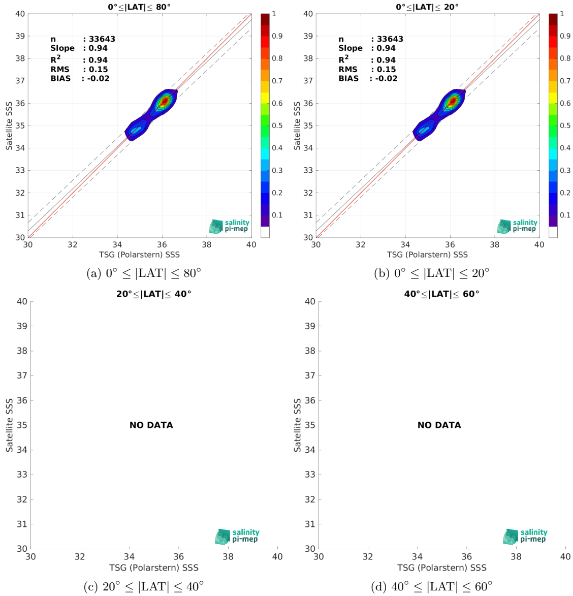
Figure 9: Contour maps of the concentration of SMAP SSS L4 OI v2 - 7 Days (ESR) SSS (y-axis) versus TSG (Polarstern) SSS (x-axis) at match-up pairs for different latitude bands. For each plot, the red line shows x=y . The black thin and dashed lines indicate a linear fit through the data cloud and the \pm 95\% confidence levels, respectively. The number match-up pairs n , the slope and R^2 coefficient of the linear fit, the root mean square (RMS) and the mean bias between satellite and in situ data are indicated for each latitude band in each plots.
