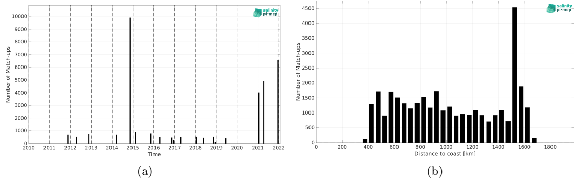
Figure 1: Number of match-ups between TSG (Polarstern) and SMAP SSS L4 OI v2 - 7 Days (ESR) SSS as a function of time (a) and as function of the distance to coast (b) over the Equatorial Ocean 10N-10S Pi-MEP region and for the full satellite product period.
