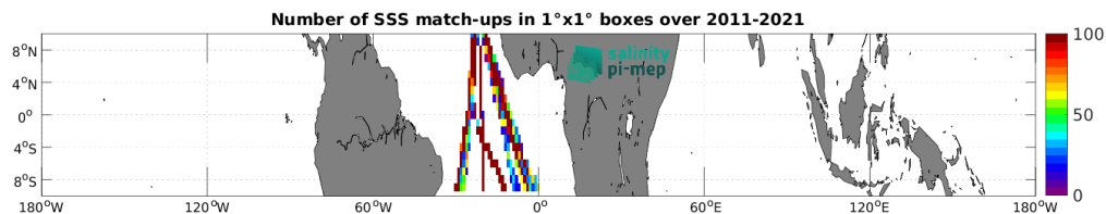
Figure 4: Number of SSS match-ups between TSG (Polarstern) SSS and the SMAP SSS L4 OI v2 - 7 Days (ESR) SSS product for the Equatorial Ocean 10N-10S Pi-MEP region over 1^\circ \times 1^\circ boxes and for the full satellite product period.
