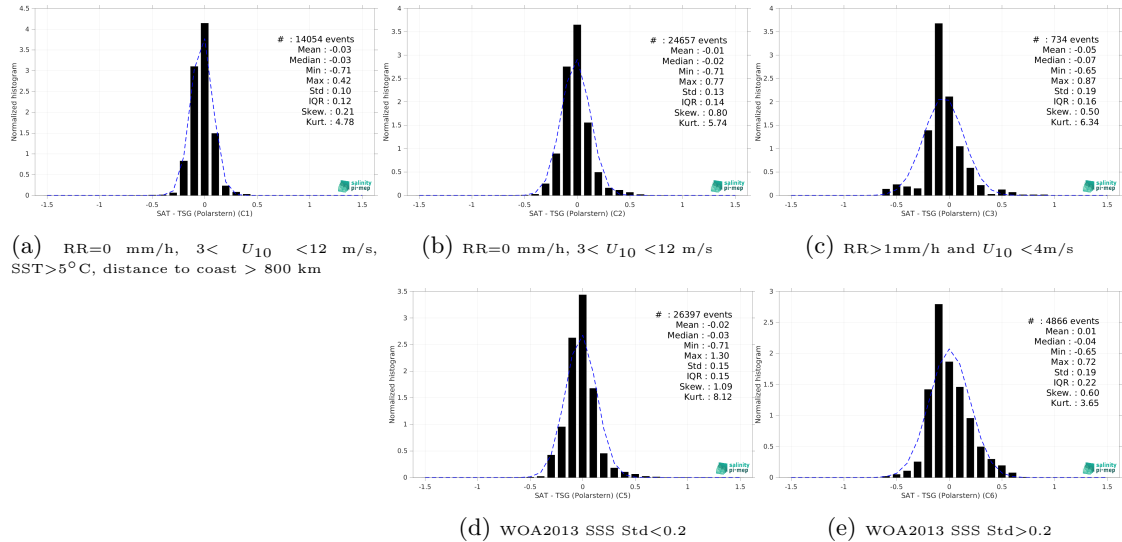
Figure 13: Normalized histogram of \Delta\text{SSS} (SMAP SSS L4 OI v2 - 7 Days (ESR) - TSG (Polarstern)) for 5 different subdatasets corresponding to: RR=0 mm/h, 3 < U_{10} < 12 m/s, SST >5^\circ\text{C} , distance to coast > 800 km (a), RR=0 mm/h, 3 < U_{10} < 12 m/s (b), RR >1 mm/h and U_{10} < 4 m/s (c), WOA2013 SSS Std <0.2 (d), WOA2013 SSS Std >0.2 (e).
