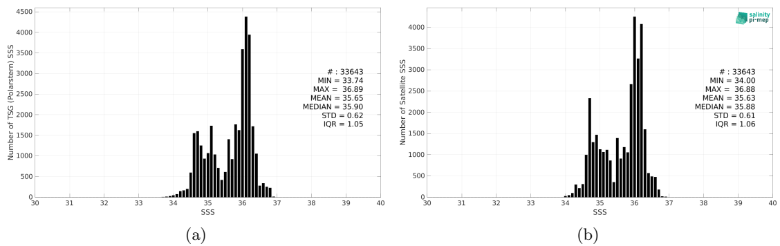
Figure 2: Histograms of SSS from TSG (Polarstern) (a) and SMAP SSS L4 OI v2 - 7 Days (ESR) (b) considering all match-up pairs per bins of 0.1 over the Equatorial Ocean 10N-10S Pi-MEP region and for the full satellite product period.
