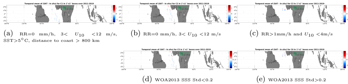
Figure 12: Temporal mean gridded over spatial boxes of size 1^\circ \times 1^\circ of \Delta SSS (SMAP SSS L4 OI v2 - 7 Days (ESR) - TSG (Polarstern)) for 5 different subdatasets corresponding to: RR=0 mm/h, 3 < U_{10} < 12 m/s, SST >5^\circ\text{C} , distance to coast > 800 km (a), RR=0 mm/h, 3 < U_{10} < 12 m/s (b), RR >1 mm/h and U_{10} < 4 m/s (c), WOA2013 SSS Std <0.2 (d), WOA2013 SSS Std >0.2 (e).
