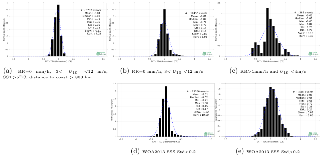
Figure 13: Normalized histogram of \Delta SSS (SMAP SSS L4 OI v2 - 7 Days (ESR) - TSG (Polarstern)) for 5 different subdatasets corresponding to: RR=0 mm/h, 3 < U_{10} < 12 m/s, SST >5^\circ\text{C} , distance to coast > 800 km (a), RR=0 mm/h, 3 < U_{10} < 12 m/s (b), RR >1 mm/h and U_{10} < 4 m/s (c), WOA2013 SSS Std <0.2 (d), WOA2013 SSS Std >0.2 (e).
