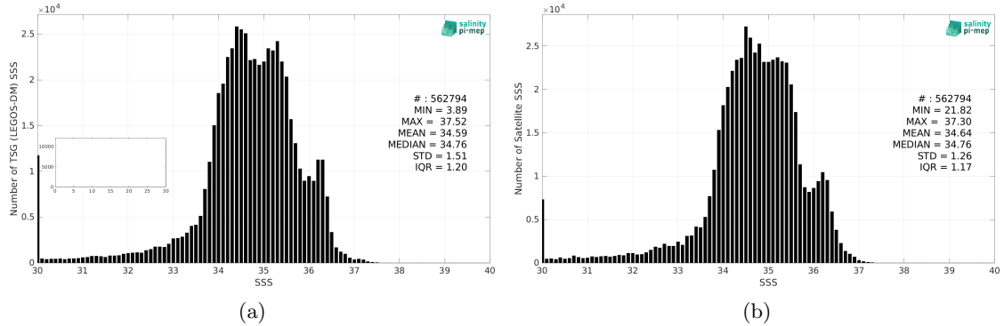
Figure 2: Histograms of SSS from TSG (LEGOS-DM) (a) and SMAP SSS L4 OI v2 - 7 Days (ESR) (b) considering all match-up pairs per bins of 0.1 over the Equatorial Ocean 10N-10S Pi-MEP region and for the full satellite product period.
