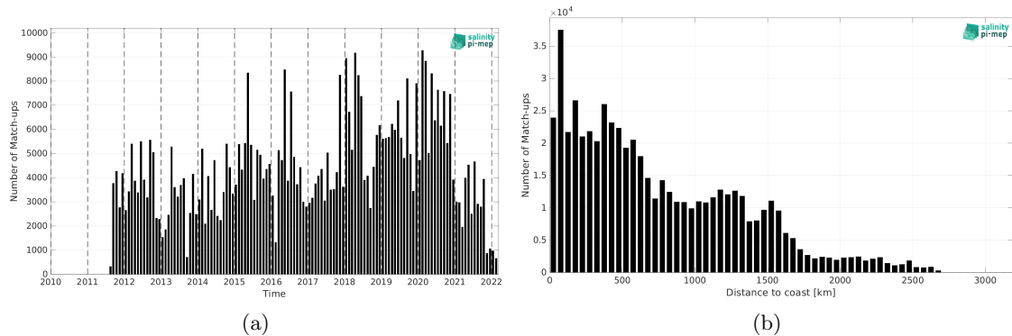
Figure 1: Number of match-ups between TSG (LEGOS-DM) and SMAP SSS L4 OI v2 - 7 Days (ESR) SSS as a function of time (a) and as function of the distance to coast (b) over the Equatorial Ocean 10N-10S Pi-MEP region and for the full satellite product period.
