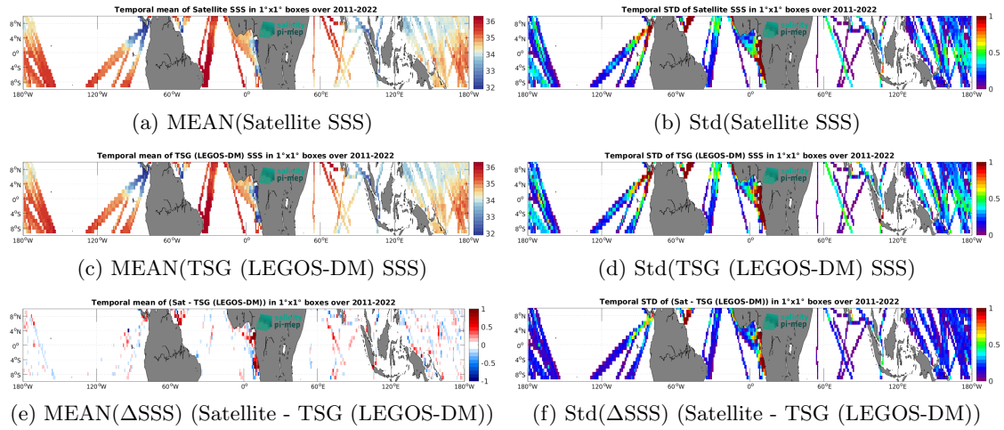
Figure 6: Temporal mean (left) and Std (right) of SSS from SMAP SSS L4 OI v2 - 7 Days (ESR) (top), TSG (LEGOS-DM) (middle), and of \Delta SSS (Satellite - TSG (LEGOS-DM)). Only match-up pairs are used to generate these maps.
