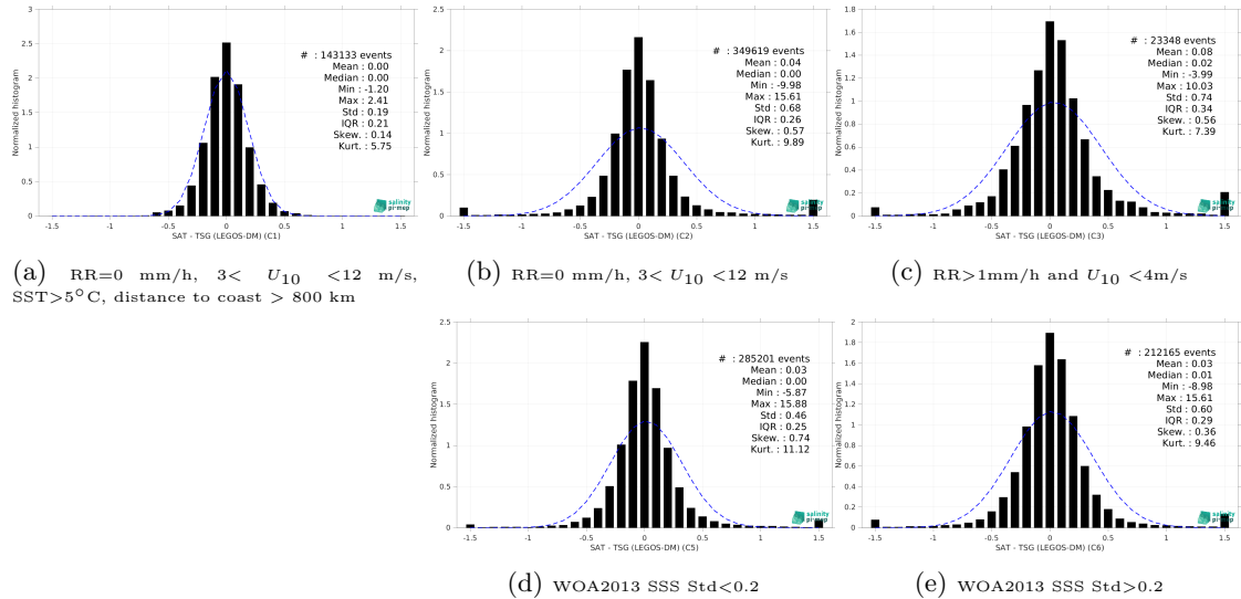
Figure 13: Normalized histogram of \Delta SSS (SMAP SSS L4 OI v2 - 7 Days (ESR) - TSG (LEGOS-DM)) for 5 different subdatasets corresponding to: RR=0 mm/h, 3 < U_{10} < 12 m/s, SST >5^\circ C, distance to coast > 800 km (a), RR=0 mm/h, 3 < U_{10} < 12 m/s (b), RR >1 mm/h and U_{10} < 4 m/s (c), WOA2013 SSS Std <0.2 (d), WOA2013 SSS Std >0.2 (e).
