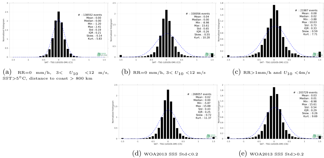
Figure 13: Normalized histogram of \Delta SSS (SMAP SSS L4 OI v2 - 7 Days (ESR) - TSG (LEGOS-DM)) for 5 different subdatasets corresponding to: RR=0 mm/h, 3 < U_{10} < 12 m/s, SST > 5^\circ C , distance to coast > 800 km (a), RR=0 mm/h, 3 < U_{10} < 12 m/s (b), RR>1mm/h and U_{10} < 4 m/s (c), WOA2013 SSS Std<0.2 (d), WOA2013 SSS Std>0.2 (e).
