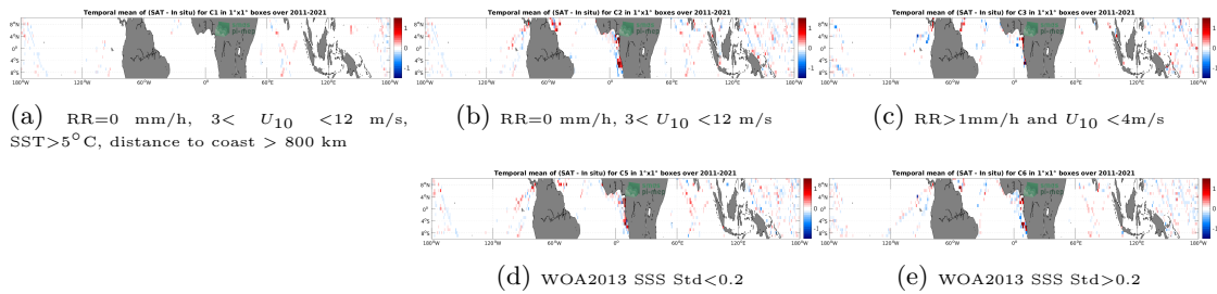
Figure 12: Temporal mean gridded over spatial boxes of size 1^\circ \times 1^\circ of \Delta SSS (SMAP SSS L4 OI v2 - 7 Days (ESR) - TSG (LEGOS-DM)) for 5 different subdatasets corresponding to:RR=0 mm/h, 3 < U_{10} < 12 m/s, SST > 5^\circ C , distance to coast > 800 km (a), RR=0 mm/h, 3 < U_{10} < 12 m/s (b), RR>1mm/h and U_{10} < 4 m/s (c), WOA2013 SSS Std<0.2 (d), WOA2013 SSS Std>0.2 (e).
