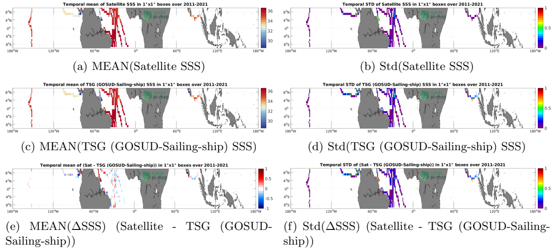
Figure 6: Temporal mean (left) and Std (right) of SSS from SMAP SSS L4 OI v2 - 7 Days (ESR) (top), TSG (GOSUD-Sailing-ship) (middle), and of \Delta SSS (Satellite - TSG (GOSUD-Sailing-ship)). Only match-up pairs are used to generate these maps.
