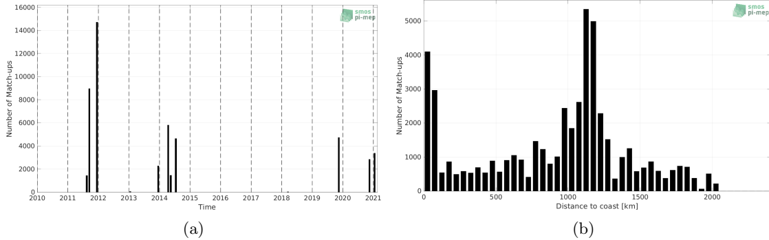
Figure 1: Number of match-ups between TSG (GOSUD-Sailing-ship) and SMAP SSS L4 OI v2 - 7 Days (ESR) SSS as a function of time (a) and as function of the distance to coast (b) over the Equatorial Ocean 10N-10S Pi-MEP region and for the full satellite product period.
