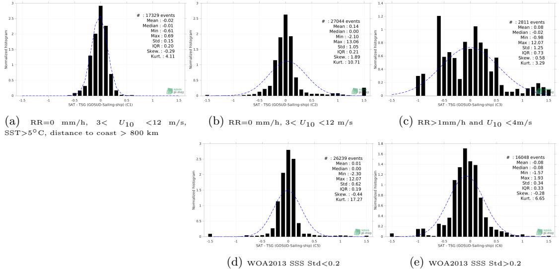
Figure 13: Normalized histogram of \Delta SSS (SMAP SSS L4 OI v2 - 7 Days (ESR) - TSG (GOSUD-Sailing-ship)) for 5 different subdatasets corresponding to: RR=0 mm/h, 3 < U_{10} < 12 m/s, SST>5°C, distance to coast > 800 km (a), RR=0 mm/h, 3 < U_{10} < 12 m/s (b), RR>1mm/h and U_{10} < 4 m/s (c), WOA2013 SSS Std<0.2 (d), WOA2013 SSS Std>0.2 (e).
