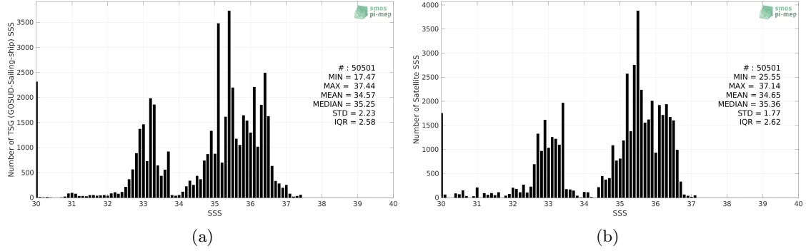
Figure 2: Histograms of SSS from TSG (GOSUD-Sailing-ship) (a) and SMAP SSS L4 OI v2 - 7 Days (ESR) (b) considering all match-up pairs per bins of 0.1 over the Equatorial Ocean 10N-10S Pi-MEP region and for the full satellite product period.
