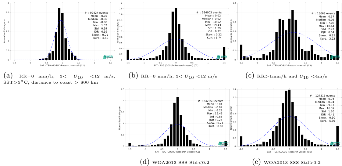
Figure 13: Normalized histogram of \Delta\text{SSS} (SMAP SSS L4 OI v2 - 7 Days (ESR) - TSG (GOSUD-Research-vessel)) for 5 different subdatasets corresponding to: RR=0 mm/h, 3 < U_{10} < 12 m/s, SST>5°C, distance to coast > 800 km (a), RR=0 mm/h, 3 < U_{10} < 12 m/s (b), RR>1mm/h and U_{10} < 4 m/s (c), WOA2013 SSS Std<0.2 (d), WOA2013 SSS Std>0.2 (e).
