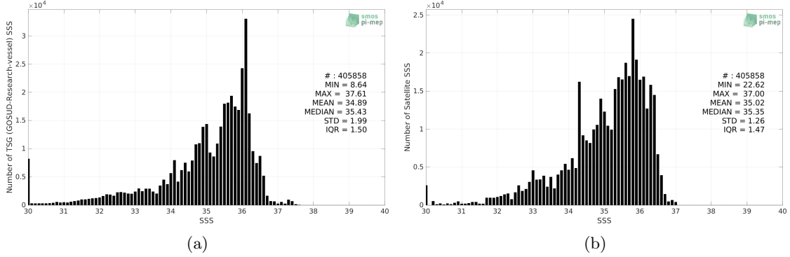
Figure 2: Histograms of SSS from TSG (GOSUD-Research-vessel) (a) and SMAP SSS L4 OI v2 - 7 Days (ESR) (b) considering all match-up pairs per bins of 0.1 over the Equatorial Ocean 10N-10S Pi-MEP region and for the full satellite product period.
