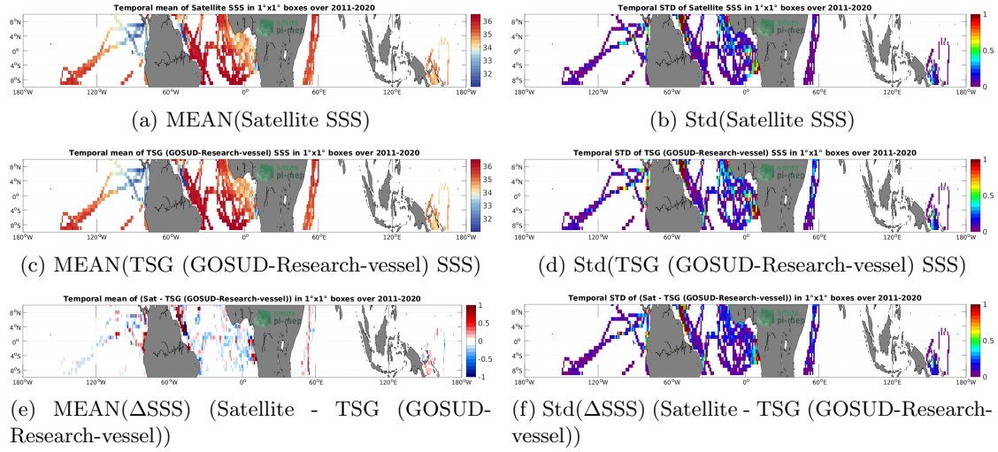
Figure 6: Temporal mean (left) and Std (right) of SSS from SMAP SSS L4 OI v2 - 7 Days (ESR) (top), TSG (GOSUD-Research-vessel) (middle), and of \Delta SSS (Satellite - TSG (GOSUD-Research-vessel)). Only match-up pairs are used to generate these maps.
