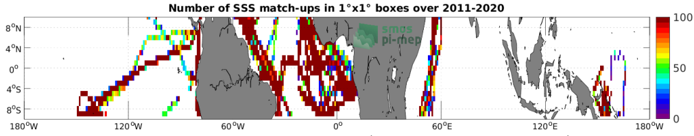
Figure 4: Number of SSS match-ups between TSG (GOSUD-Research-vessel) SSS and the SMAP SSS L4 OI v2 - 7 Days (ESR) SSS product for the Equatorial Ocean 10N-10S Pi-MEP region over 1^\circ \times 1^\circ boxes and for the full satellite product period.
