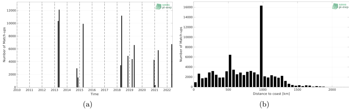
Figure 1: Number of match-ups between TSG (CSIC-UTM) and SMAP SSS L4 OI v2 - 7 Days (ESR) SSS as a function of time (a) and as function of the distance to coast (b) over the Equatorial Ocean 10N-10S Pi-MEP region and for the full satellite product period.
