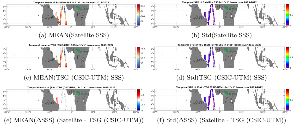
Figure 6: Temporal mean (left) and Std (right) of SSS from SMAP SSS L4 OI v2 - 7 Days (ESR) (top), TSG (CSIC-UTM) (middle), and of \Delta SSS (Satellite - TSG (CSIC-UTM)). Only match-up pairs are used to generate these maps.
