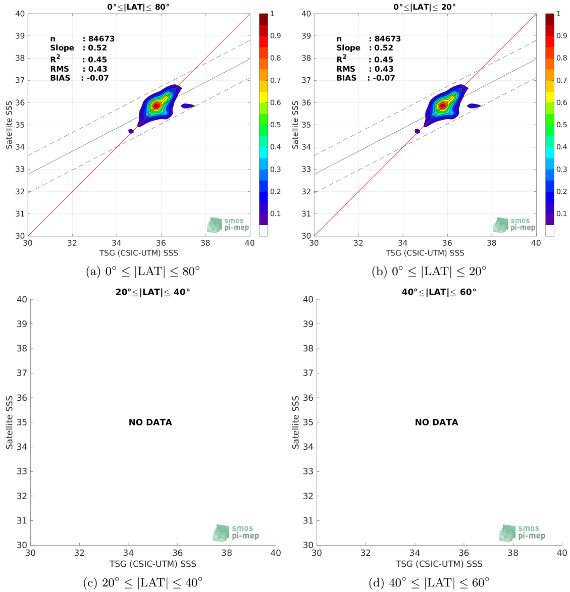
Figure 9: Contour maps of the concentration of SMAP SSS L4 OI v2 - 7 Days (ESR) SSS (y-axis) versus TSG (CSIC-UTM) SSS (x-axis) at match-up pairs for different latitude bands. For each plot, the red line shows x=y . The black thin and dashed lines indicate a linear fit through the data cloud and the \pm 95\% confidence levels, respectively. The number match-up pairs n , the slope and R^2 coefficient of the linear fit, the root mean square (RMS) and the mean bias between satellite and in situ data are indicated for each latitude band in each plots.
