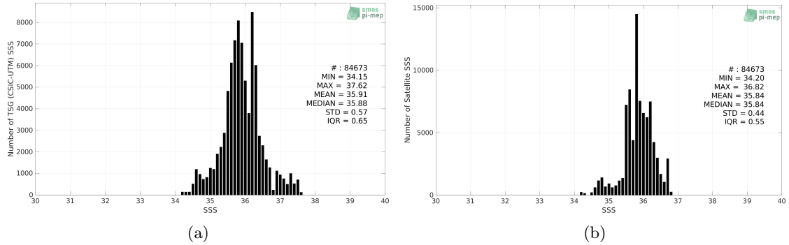
Figure 2: Histograms of SSS from TSG (CSIC-UTM) (a) and SMAP SSS L4 OI v2 - 7 Days (ESR) (b) considering all match-up pairs per bins of 0.1 over the Equatorial Ocean 10N-10S Pi-MEP region and for the full satellite product period.
