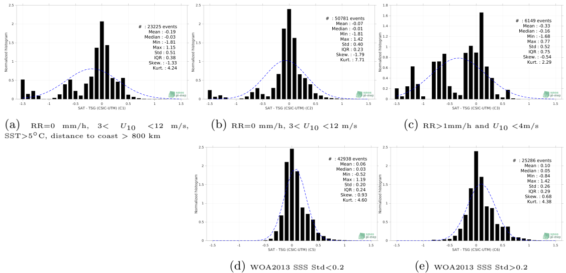
Figure 13: Normalized histogram of \Delta SSS (SMAP SSS L4 OI v2 - 7 Days (ESR) - TSG (CSIC-UTM)) for 5 different subdatasets corresponding to: RR=0 mm/h, 3 < U_{10} < 12 m/s, SST>5°C, distance to coast > 800 km (a), RR=0 mm/h, 3 < U_{10} < 12 m/s (b), RR>1mm/h and U_{10} < 4 m/s (c), WOA2013 SSS Std<0.2 (d), WOA2013 SSS Std>0.2 (e).
