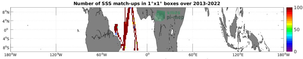
Figure 4: Number of SSS match-ups between TSG (CSIC-UTM) SSS and the SMAP SSS L4 OI v2 - 7 Days (ESR) SSS product for the Equatorial Ocean 10N-10S Pi-MEP region over 1^\circ \times 1^\circ boxes and for the full satellite product period.
