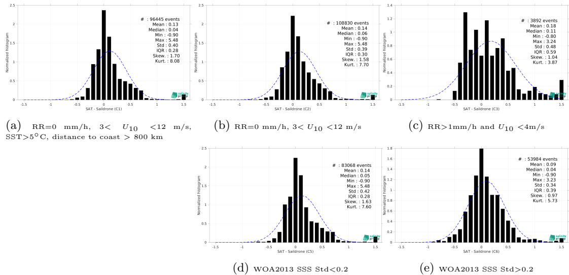
Figure 13: Normalized histogram of \Delta SSS (SMAP SSS L4 OI v2 - 7 Days (ESR) - Saildrone) for 5 different subdatasets corresponding to: RR=0 mm/h, 3 < U_{10} < 12 m/s, SST >5^\circ\text{C} , distance to coast > 800 km (a), RR=0 mm/h, 3 < U_{10} < 12 m/s (b), RR >1 mm/h and U_{10} < 4 m/s (c), WOA2013 SSS Std <0.2 (d), WOA2013 SSS Std >0.2 (e).
