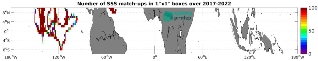
Figure 4: Number of SSS match-ups between Saildrone SSS and the SMAP SSS L4 OI v2 - 7 Days (ESR) SSS product for the Equatorial Ocean 10N-10S Pi-MEP region over 1^\circ \times 1^\circ boxes and for the full satellite product period.
