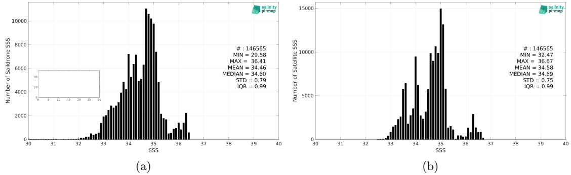
Figure 2: Histograms of SSS from Saildrone (a) and SMAP SSS L4 OI v2 - 7 Days (ESR) (b) considering all match-up pairs per bins of 0.1 over the Equatorial Ocean 10N-10S Pi-MEP region and for the full satellite product period.
