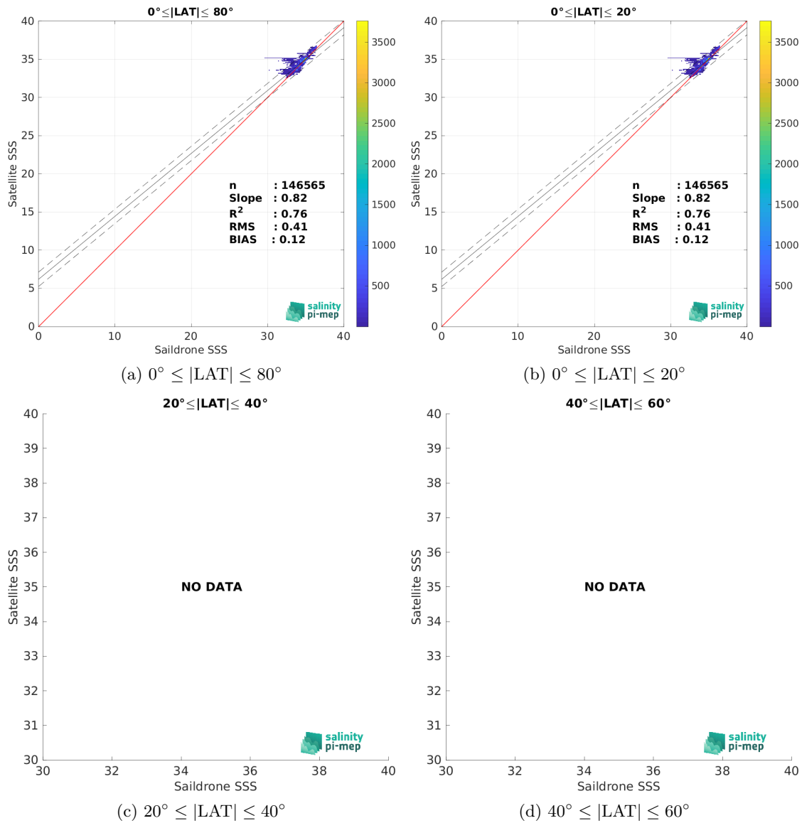
Figure 9: Contour maps of the concentration of SMAP SSS L4 OI v2 - 7 Days (ESR) SSS (y-axis) versus Sairdrone SSS (x-axis) at match-up pairs for different latitude bands. For each plot, the red line shows x=y . The black thin and dashed lines indicate a linear fit through the data cloud and the \pm 95\% confidence levels, respectively. The number match-up pairs n , the slope and R^2 coefficient of the linear fit, the root mean square (RMS) and the mean bias between satellite and in situ data are indicated for each latitude band in each plots.
