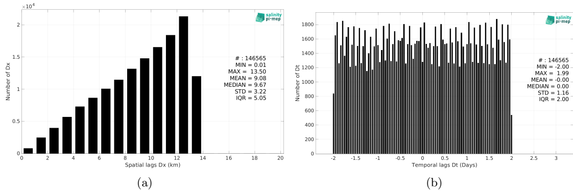
Figure 5: Histograms of the spatial (a) and temporal (b) lags between the location/time of the Saildrone measurement and the date of the corresponding SMAP SSS L4 OI v2 - 7 Days (ESR) SSS pixel.
