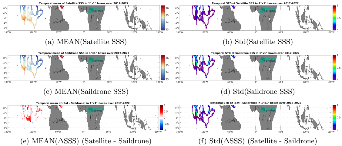
Figure 6: Temporal mean (left) and Std (right) of SSS from SMAP SSS L4 OI v2 - 7 Days (ESR) (top), Saildrone (middle), and of \Delta SSS (Satellite - Saildrone). Only match-up pairs are used to generate these maps.
