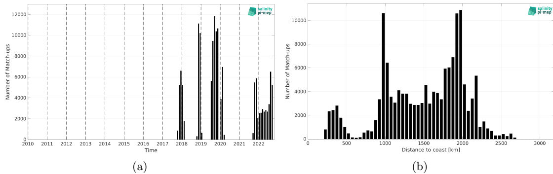
Figure 1: Number of match-ups between Saildrone and SMAP SSS L4 OI v2 - 7 Days (ESR) SSS as a function of time (a) and as function of the distance to coast (b) over the Equatorial Ocean 10N-10S Pi-MEP region and for the full satellite product period.
