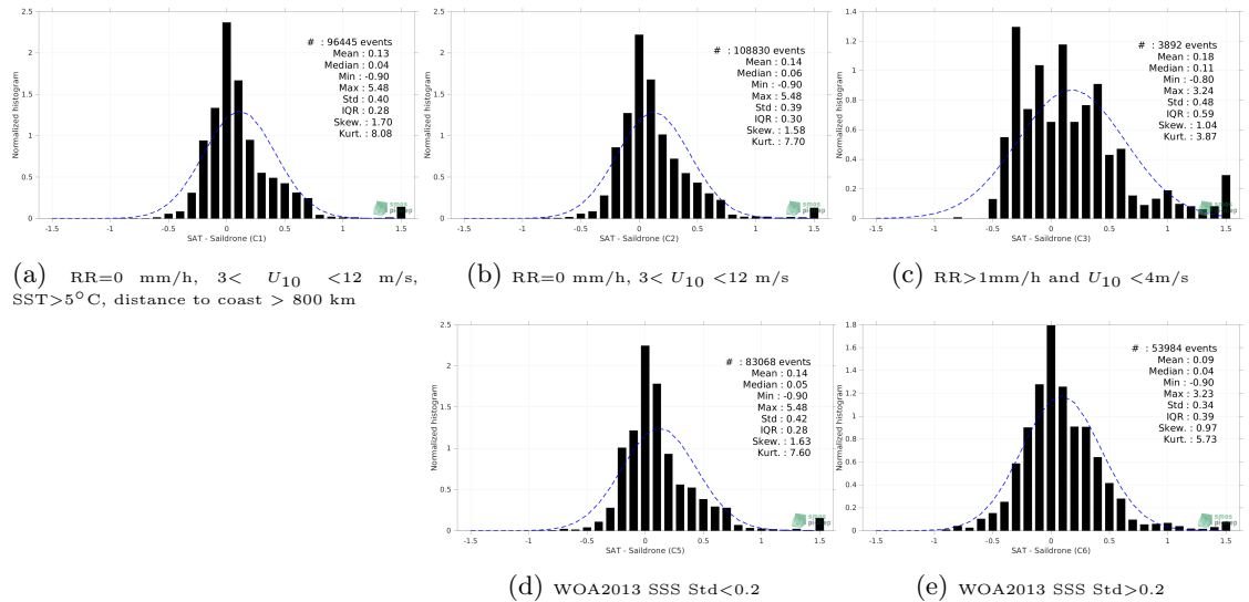
Figure 13: Normalized histogram of \Delta SSS (SMAP SSS L4 OI v2 - 7 Days (ESR) - Saildrone) for 5 different subdatasets corresponding to: RR=0 mm/h, 3 < U_{10} < 12 m/s, SST >5^\circ\text{C} , distance to coast > 800 km (a), RR=0 mm/h, 3 < U_{10} < 12 m/s (b), RR >1 mm/h and U_{10} < 4 m/s (c), WOA2013 SSS Std <0.2 (d), WOA2013 SSS Std >0.2 (e).
