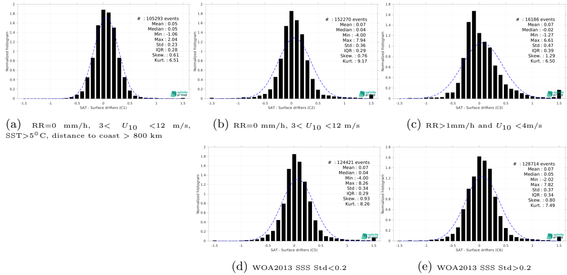
Figure 12: Normalized histogram of \Delta SSS (SMAP SSS L4 OI v2 - 7 Days (ESR) - Surface drifters) for 5 different subdatasets corresponding to: RR=0 mm/h, 3 < U_{10} < 12 m/s, SST >5^\circ C, distance to coast > 800 km (a), RR=0 mm/h, 3 < U_{10} < 12 m/s (b), RR >1 mm/h and U_{10} < 4 m/s (c), WOA2013 SSS Std <0.2 (d), WOA2013 SSS Std >0.2 (e).
