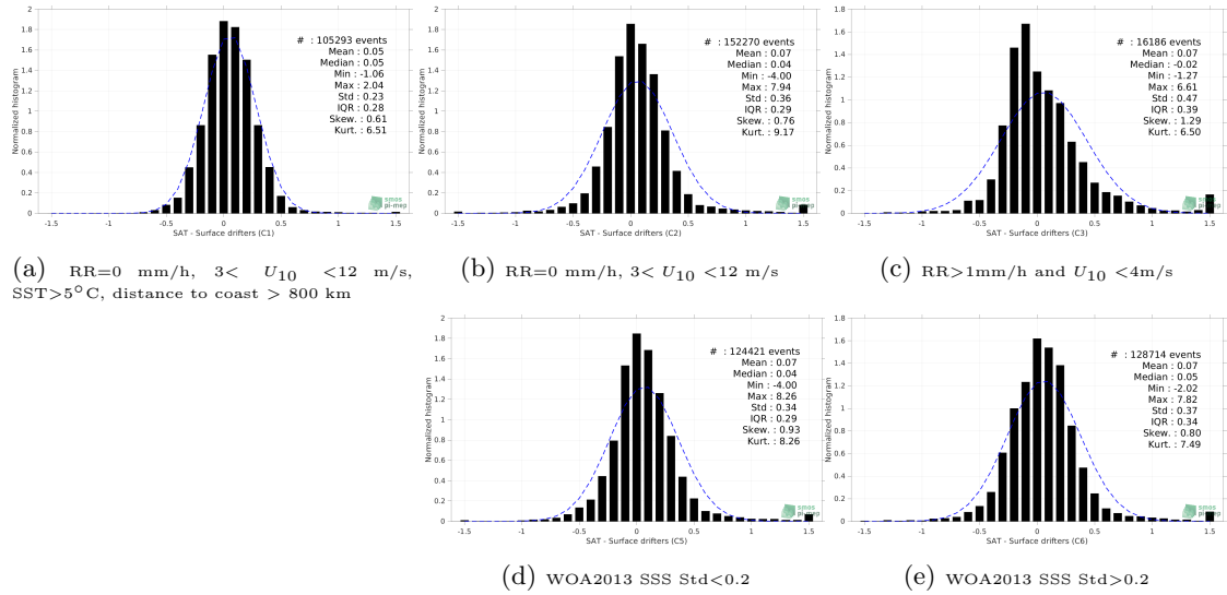
Figure 12: Normalized histogram of \Delta SSS (SMAP SSS L4 OI v2 - 7 Days (ESR) - Surface drifters) for 5 different subdatasets corresponding to: RR=0 mm/h, 3 < U_{10} < 12 m/s, SST > 5^\circ C , distance to coast > 800 km (a), RR=0 mm/h, 3 < U_{10} < 12 m/s (b), RR > 1 mm/h and U_{10} < 4 m/s (c), WOA2013 SSS Std < 0.2 (d), WOA2013 SSS Std > 0.2 (e).
