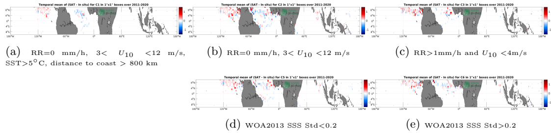
Figure 11: Temporal mean gridded over spatial boxes of size 1^\circ \times 1^\circ of \Delta SSS (SMAP SSS L4 OI v2 - 7 Days (ESR) - Surface drifters) for 5 different subdatasets corresponding to: RR=0 mm/h, 3 < U_{10} < 12 m/s, SST > 5^\circ C , distance to coast > 800 km (a), RR=0 mm/h, 3 < U_{10} < 12 m/s (b), RR > 1 mm/h and U_{10} < 4 m/s (c), WOA2013 SSS Std < 0.2 (d), WOA2013 SSS Std > 0.2 (e).
