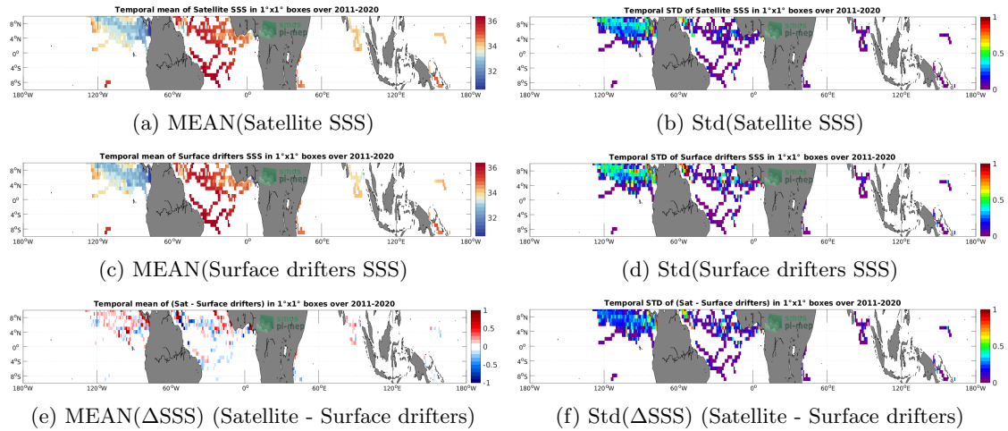
Figure 5: Temporal mean (left) and Std (right) of SSS from SMAP SSS L4 OI v2 - 7 Days (ESR) (top), Surface drifters (middle), and of \Delta SSS (Satellite - Surface drifters). Only match-up pairs are used to generate these maps.
