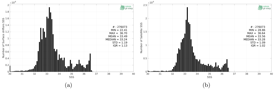
Figure 2: Histograms of SSS from Surface drifters (a) and SMAP SSS L4 OI v2 - 7 Days (ESR) (b) considering all match-up pairs per bins of 0.1 over the Equatorial Ocean 10N-10S Pi-MEP region and for the full satellite product period.
